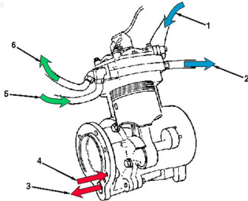
Compressor Coolant, Lubricant and Airflow
