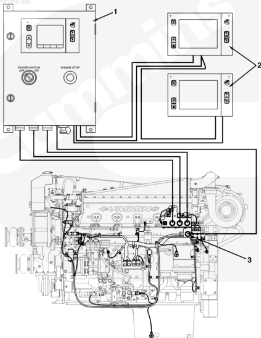
Marine C Command Elite Plus Panel System
