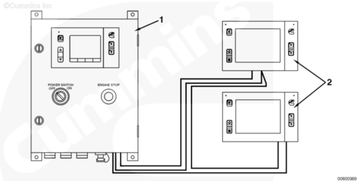
Marine C Command Elite Panel System
