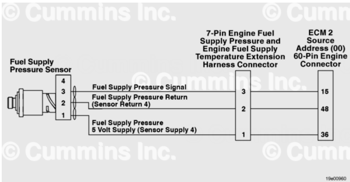
QSK38 CM2150 Power Generation/QSK38 CM2150 Power Generation (Military Application) - Fuel Delivery Pressure Sensor Circuit
