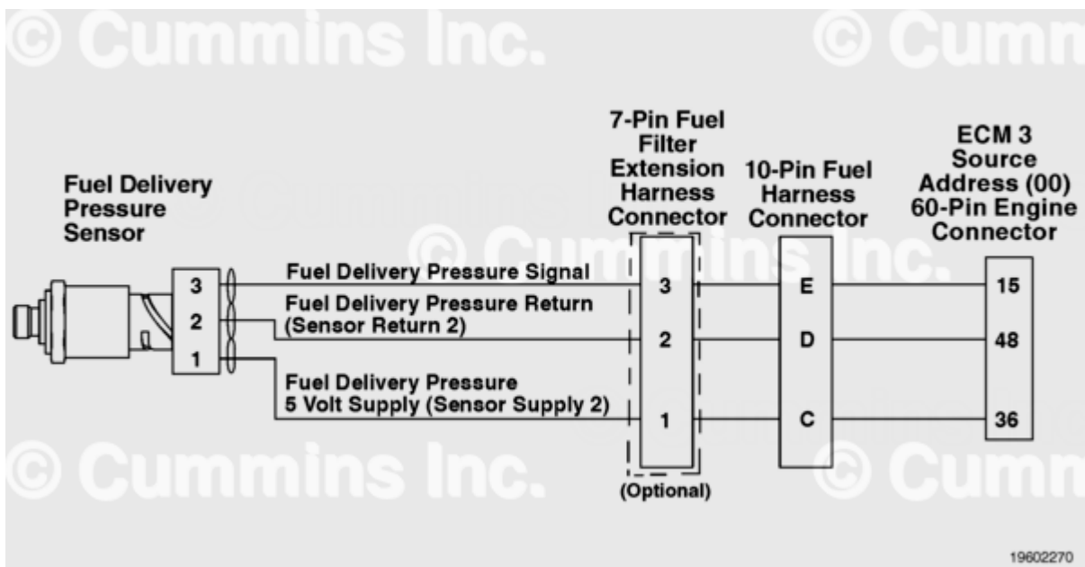
QSK50 CM2150 Power Generation without Advanced Engine Monitoring/QSK50 CM2150 Power Generation with Advanced Engine Monitoring and QSK60 CM2150 Power Generation - Fuel Delivery Pressure Sensor Circuit
