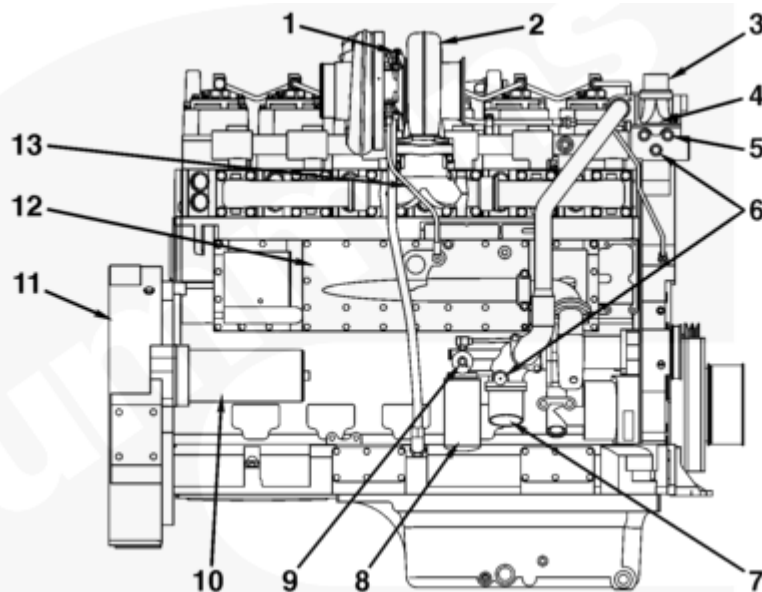
QSK19 CM2150 Modular Common Rail System Industrial and Power Generation, Exhaust Side View
