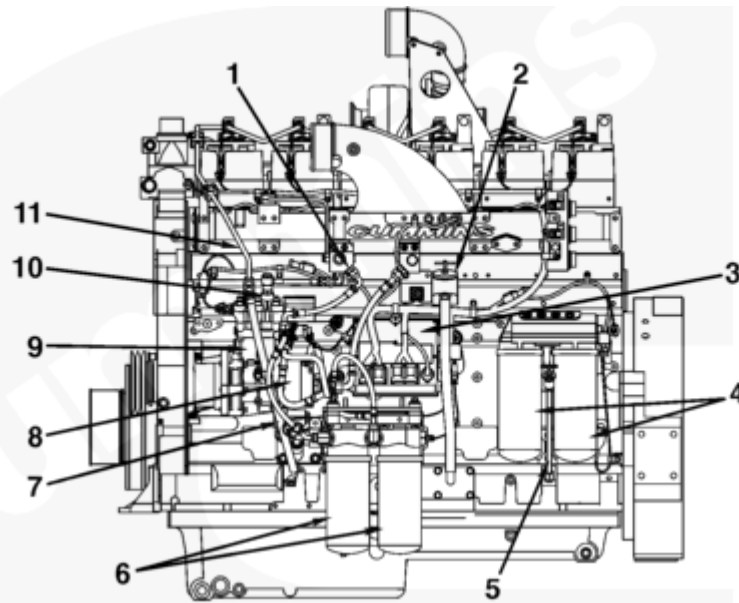
QSK19 CM2150 Modular Common Rail System Industrial and Power Generation, Intake Side View
