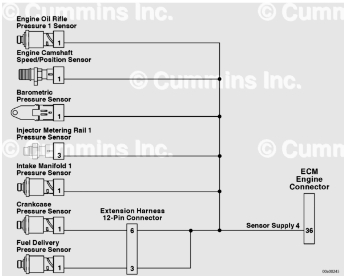
QSK19 CM2150 Marine - Sensor Supply 4 Circuit
