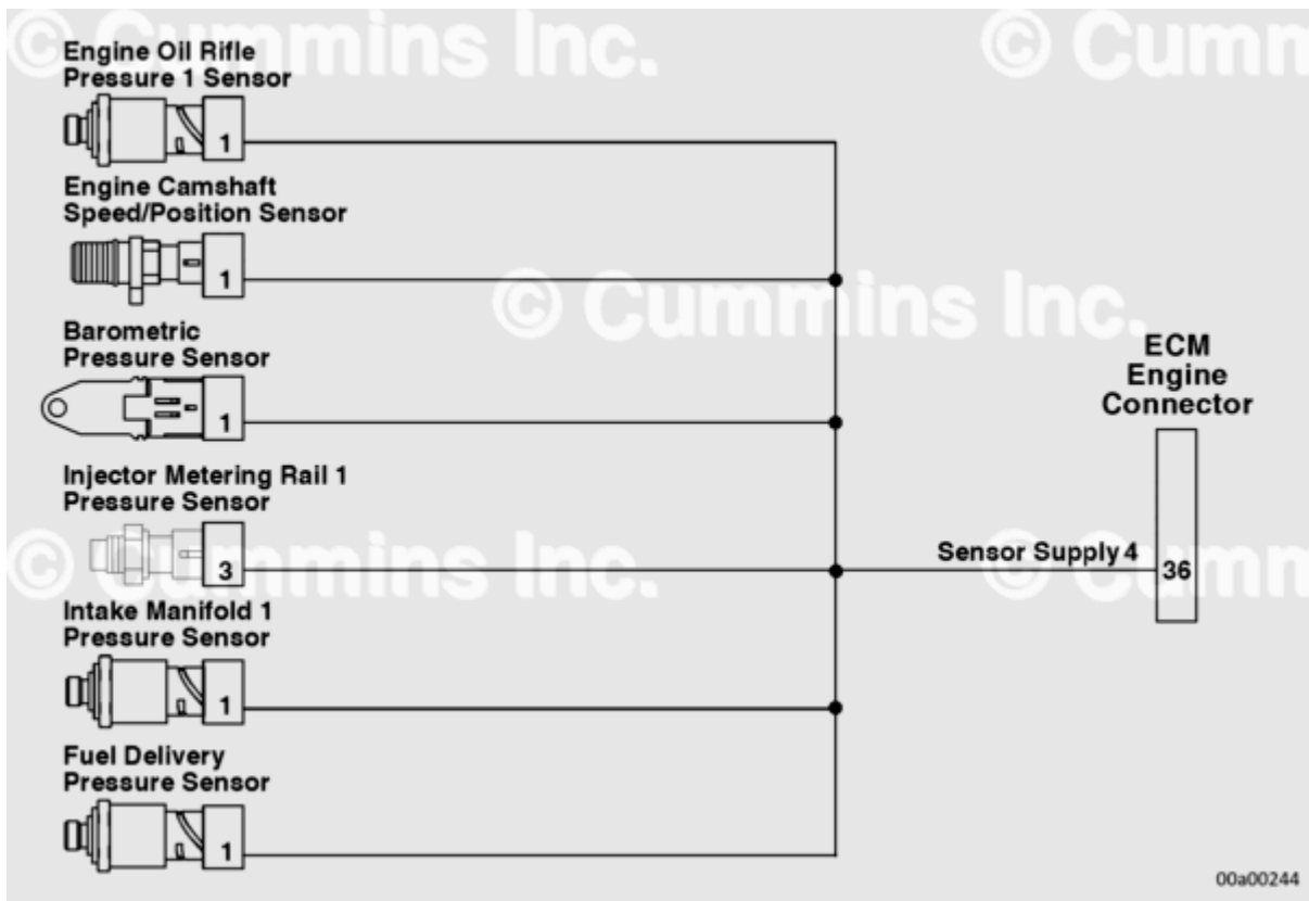
QSK19 CM2150 Marine - Sensor Supply 4 Circuit
