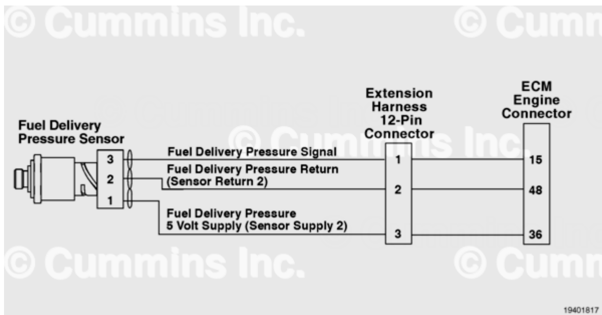
QSK19 CM2150 Marine- Fuel Delivery Pressure Sensor Circuit
