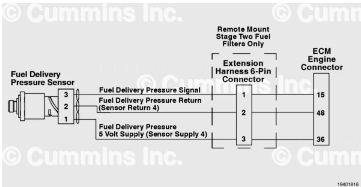
QSK19 CM2150 Industrial - Fuel Delivery Pressure Sensor Circuit
