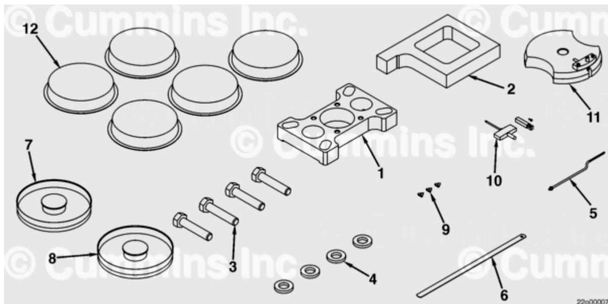
Counterbore Cutter Kit, Part Number 2892436
