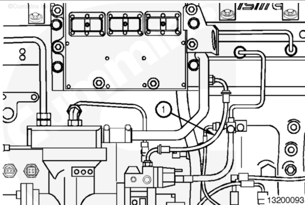
Fig. 1, Flexible Steel-Braided Fuel Line
