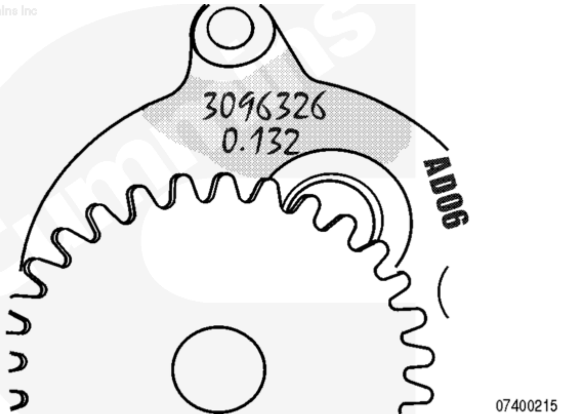
Fig. 7, QSK19 Lubricating Oil Pump with Yellow Dykem Mark, Part Number, End Clearance, and Date Code Stamped in White
