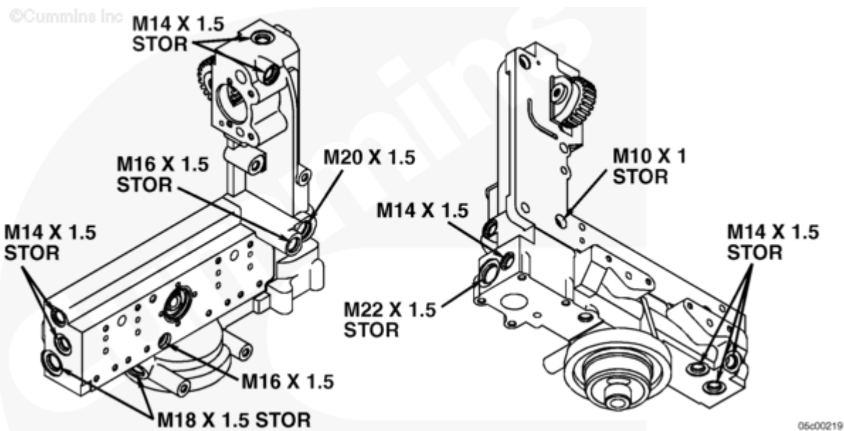
Figure 1, Integrated Fuel System Module (IFSM) Port Locations.
