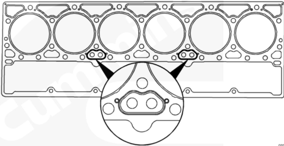
Fig. 3, Improved Steel Carrier Water Grommet
