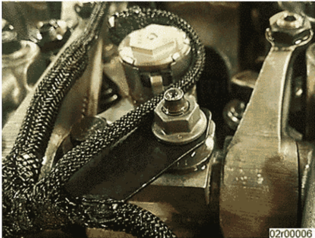
Figure 2, Mounting Tab Secured to Studed Rocker Shaft Capscrew
