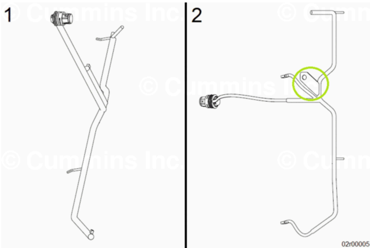
Figure 1, Number 1 on Left: Previous Design. Number 2 on Right: New Design Including Mounting Tab.
