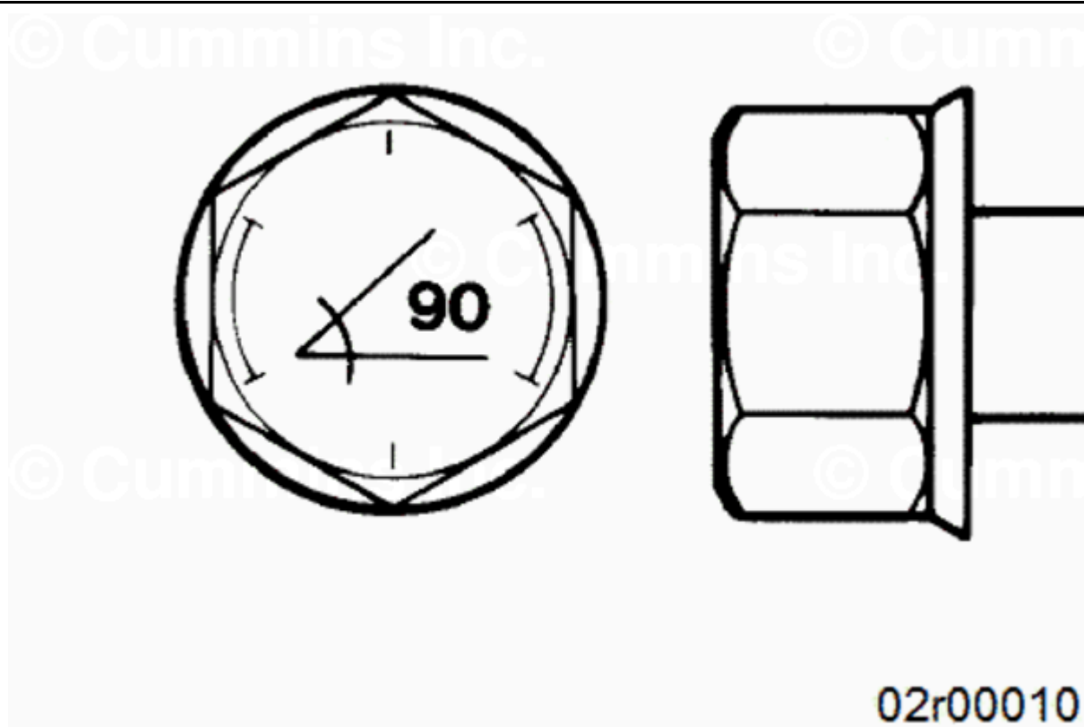
Figure 2, Obsolete Flange Head Capscrew
