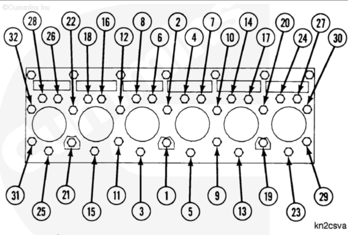
Figure 4, Capscrew Torque Sequence
