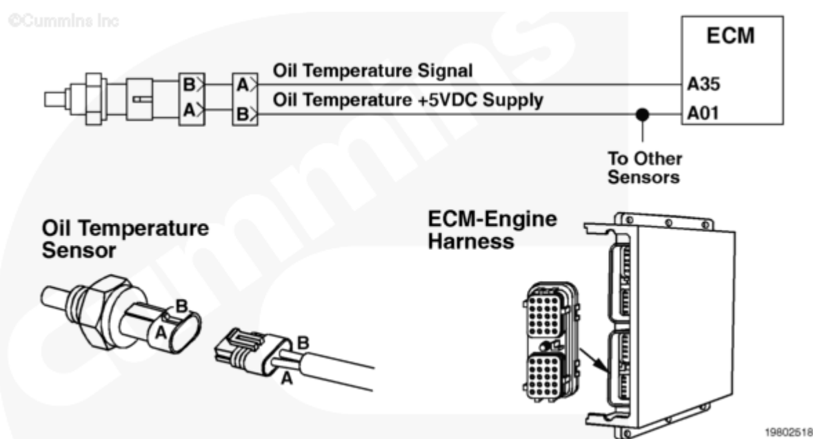
Oil Temperature Sensor Circuit
