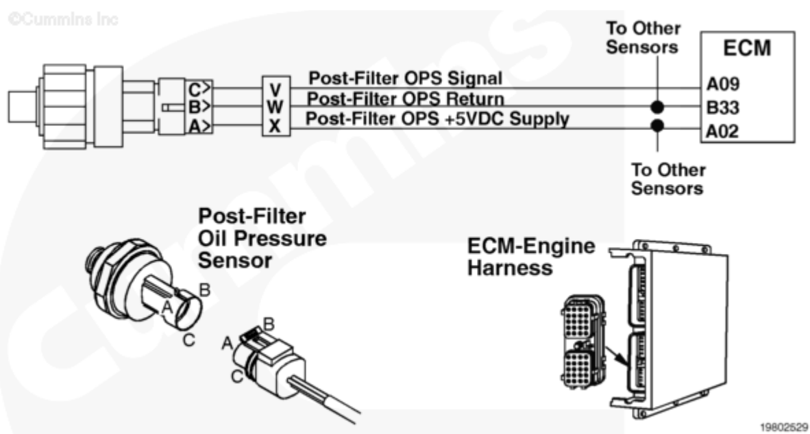
Post-Filter Oil Pressure Sensor Circuit
