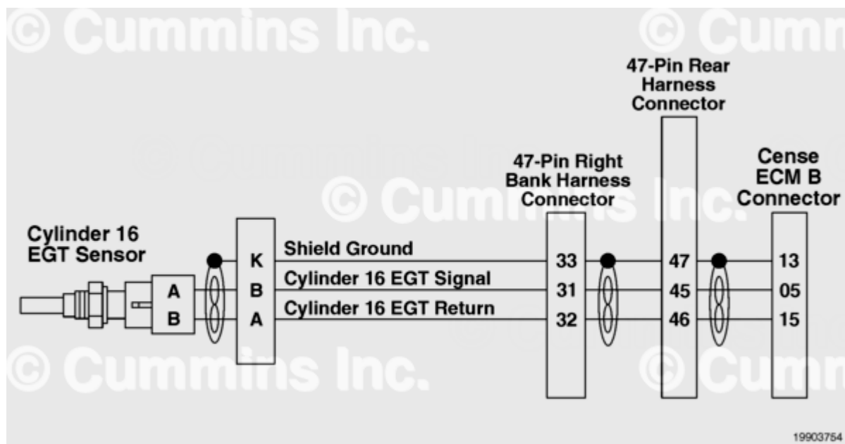
Exhaust Gas Temperature Sensor Circuit Cylinder 16
