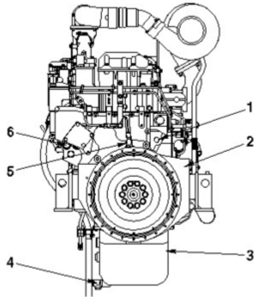
Rear View - Industrial and Power Generation
