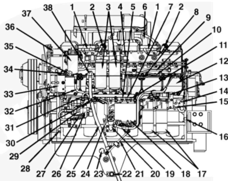
Left Side - Industrial
