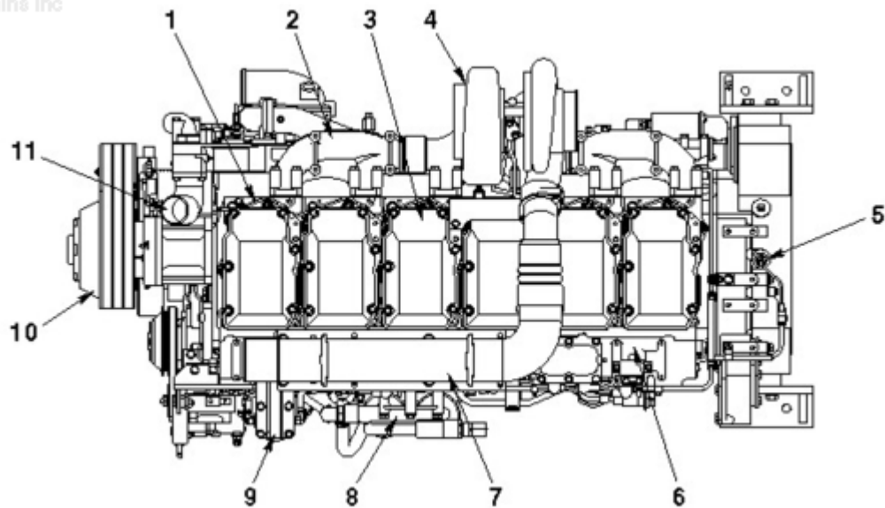
Top View - Industrial and Power Generation
