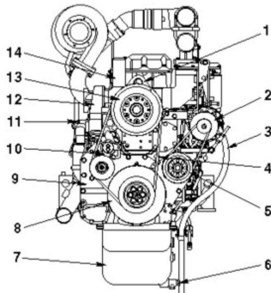
Front View - Industrial and Power Generation
