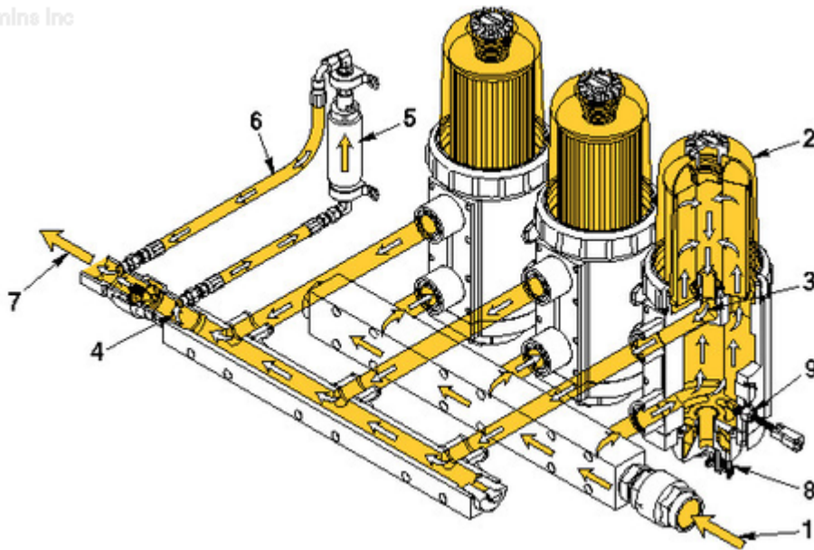
Stage 1 Triple Fuel Filter
