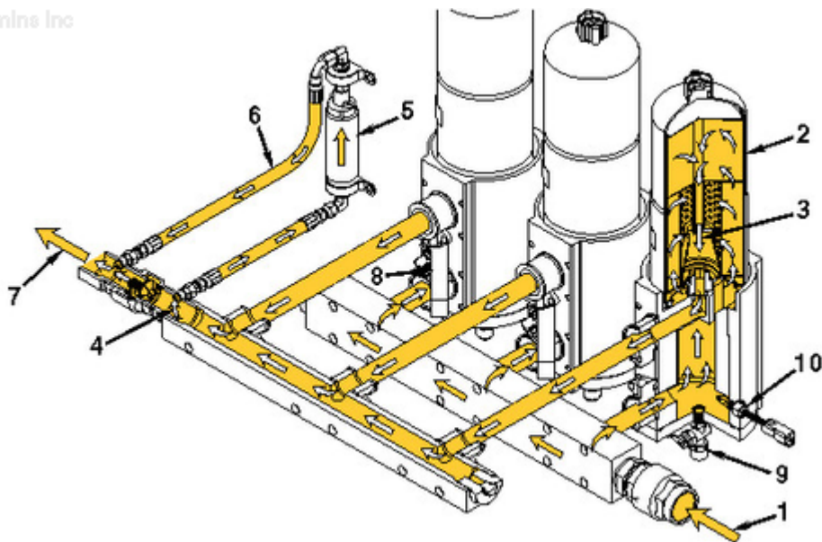
Stage 1 Triplex Fuel Filters
