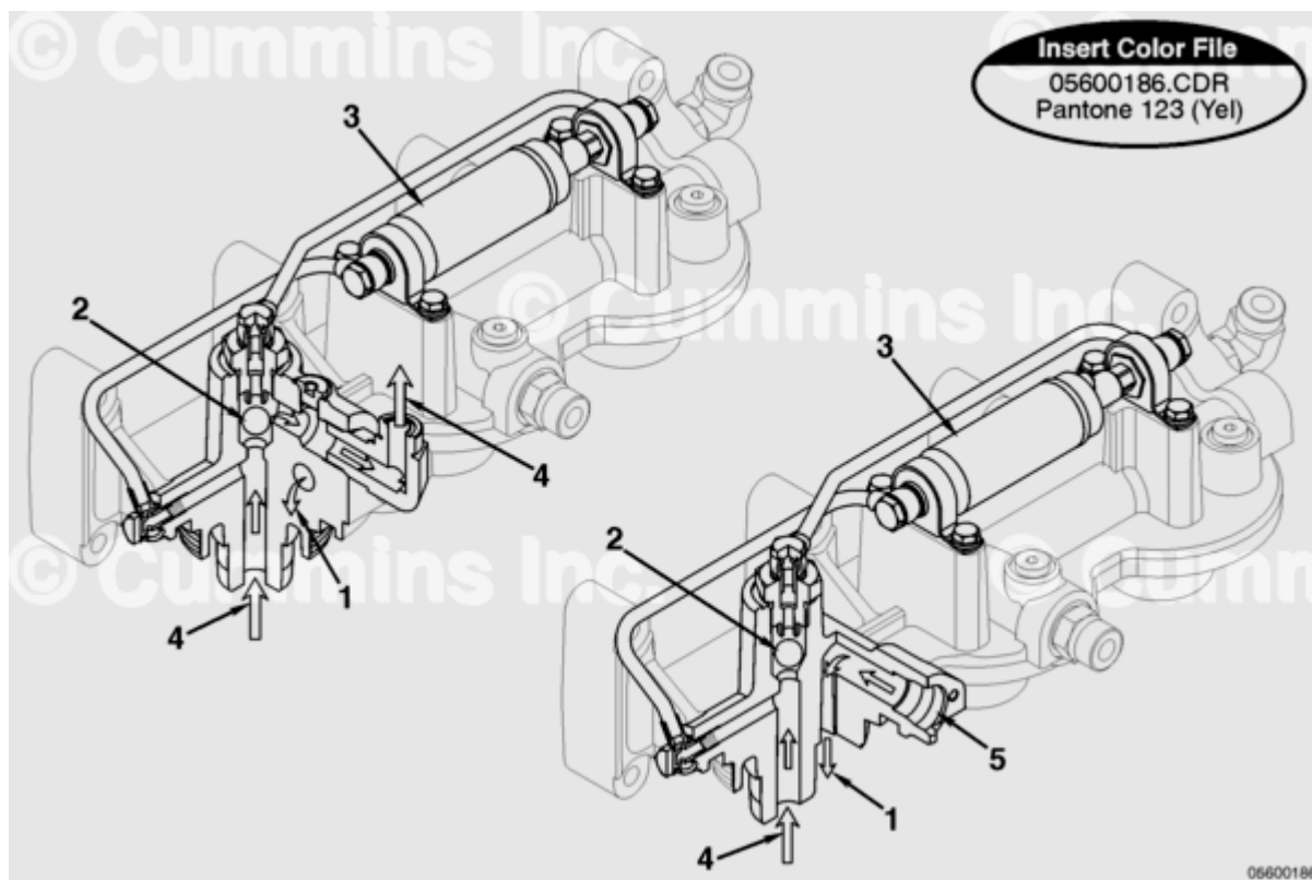
First Stage Fuel Filter Head - Check Valve Open
