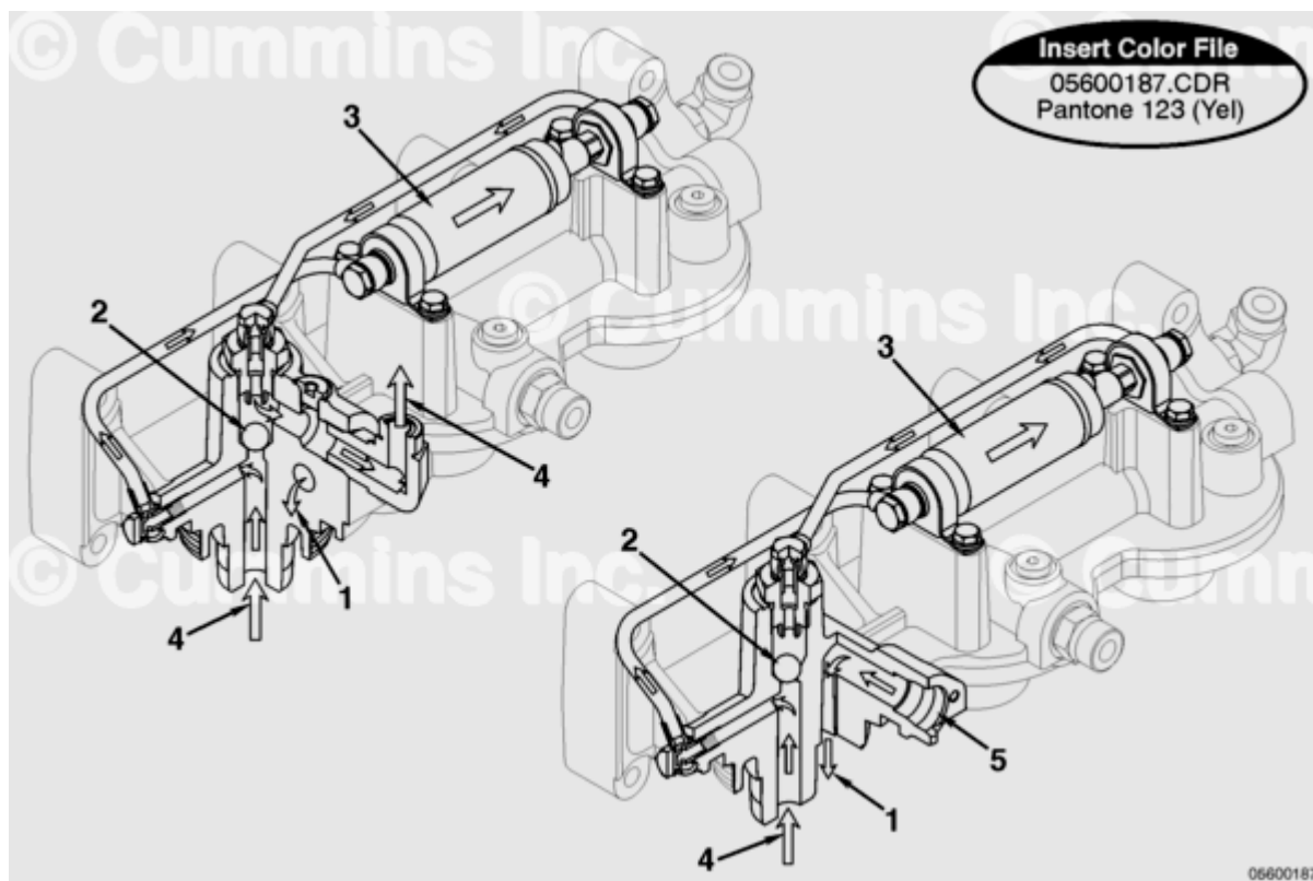
First Stage Fuel Filter Head - Check Valve Closed (Cranking)
