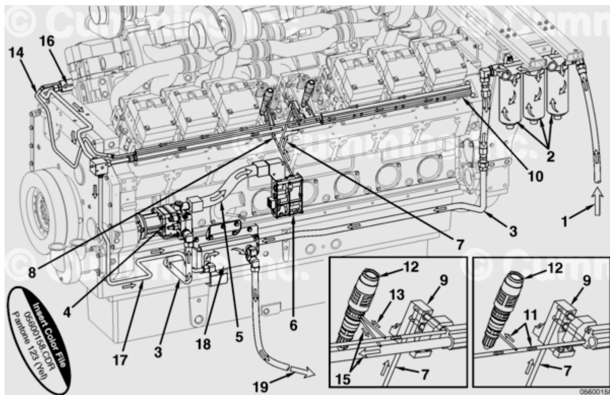
QSK60 Fuel System - Marine
