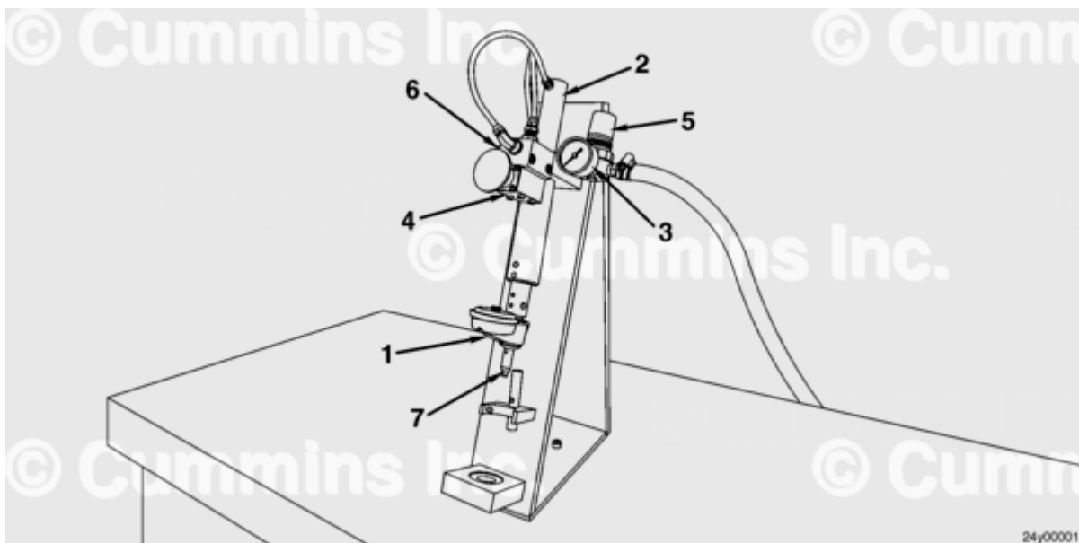
Figure 1: Injector Inspection Gauge, Part Number 3375209
