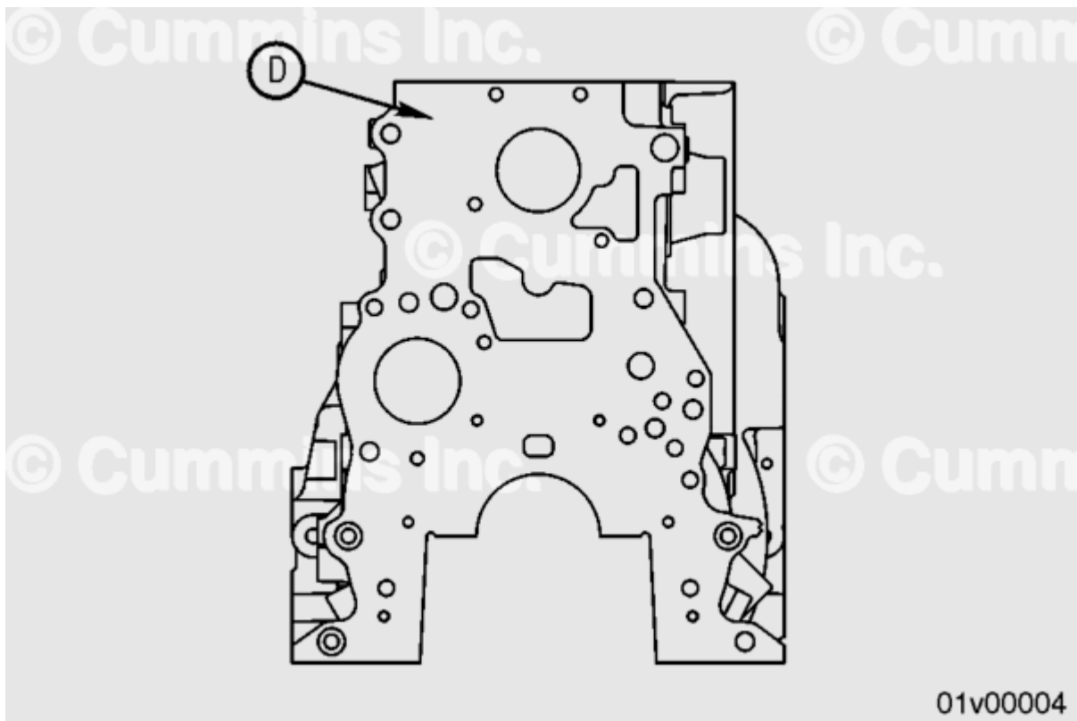
Rear View - QSB, ISB, ISD, ISBe, and B
