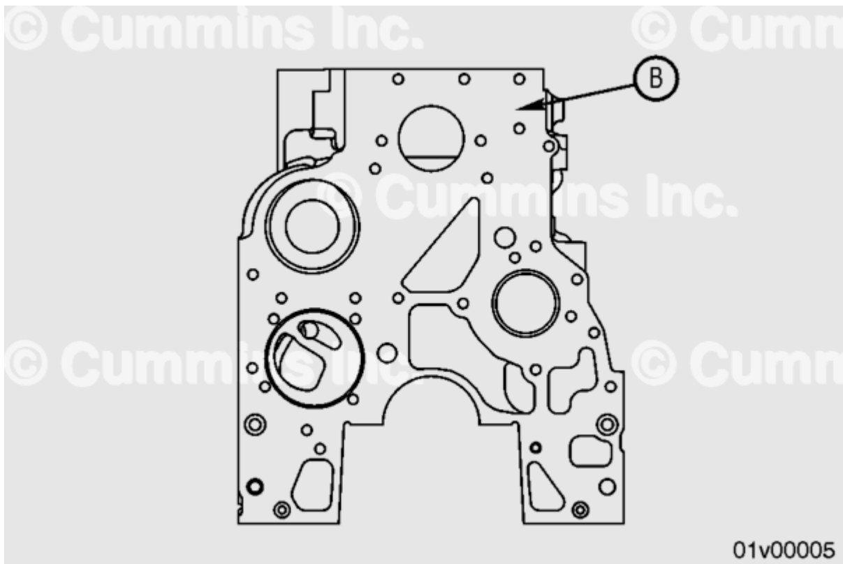
Front View - QSB, ISB, ISD, ISBe, and B
