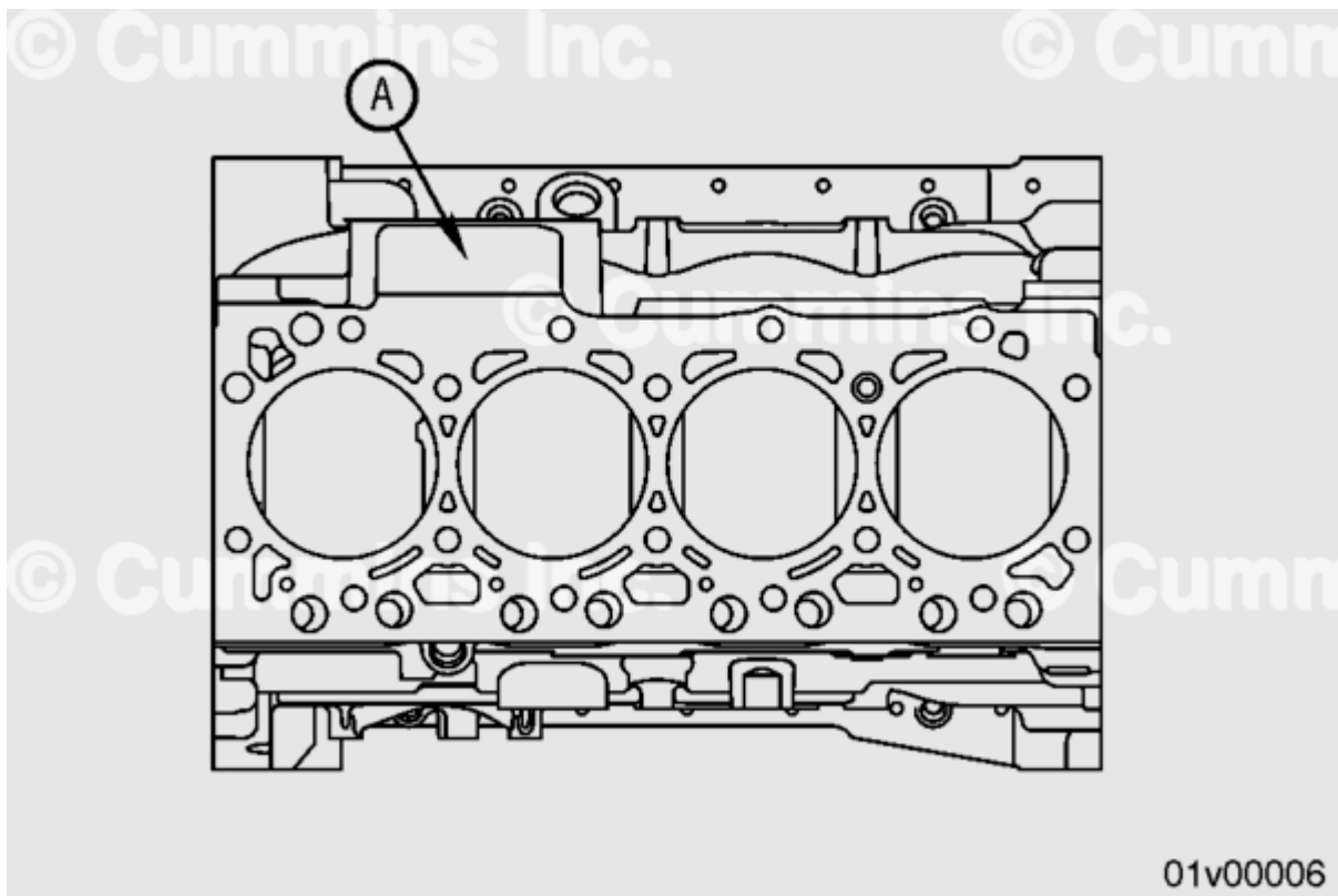
Top View - ISB, ISD, ISBe, and B-4 Cylinder
