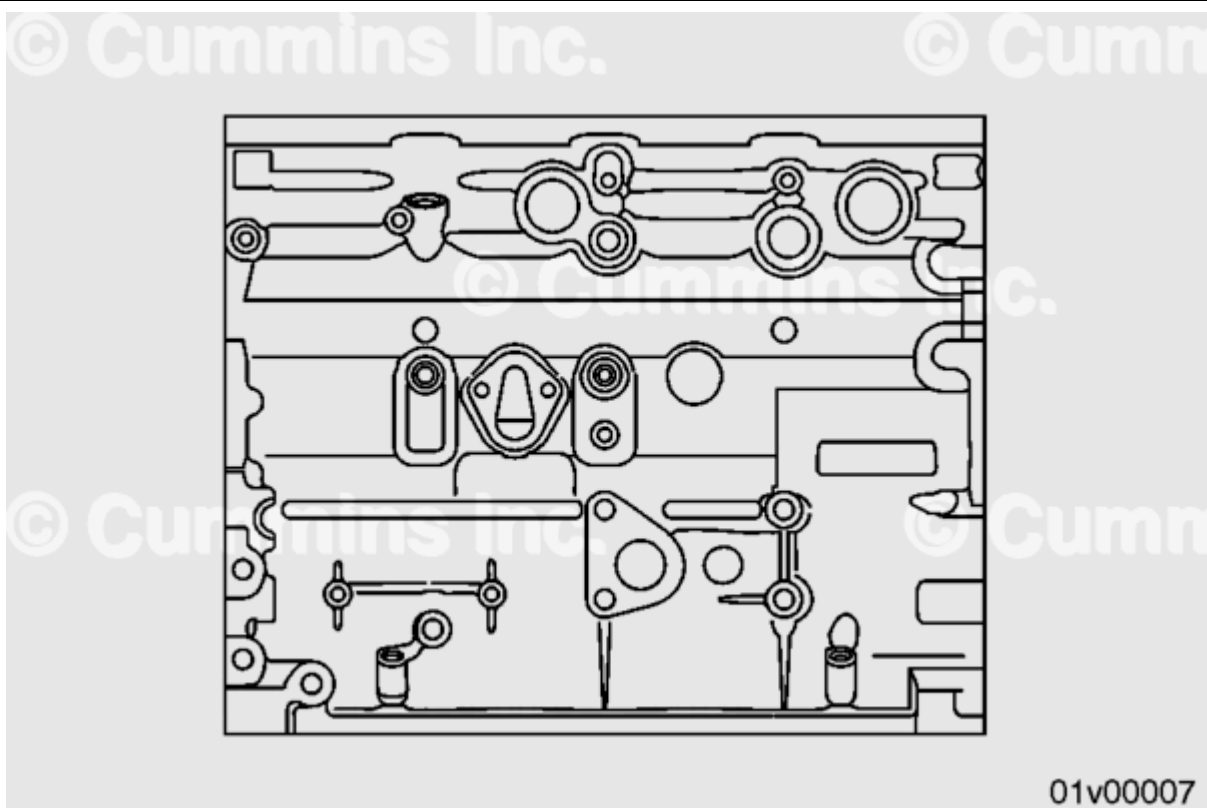
Left Side View - ISB, ISD, ISBe, and B-4 Cylinder
