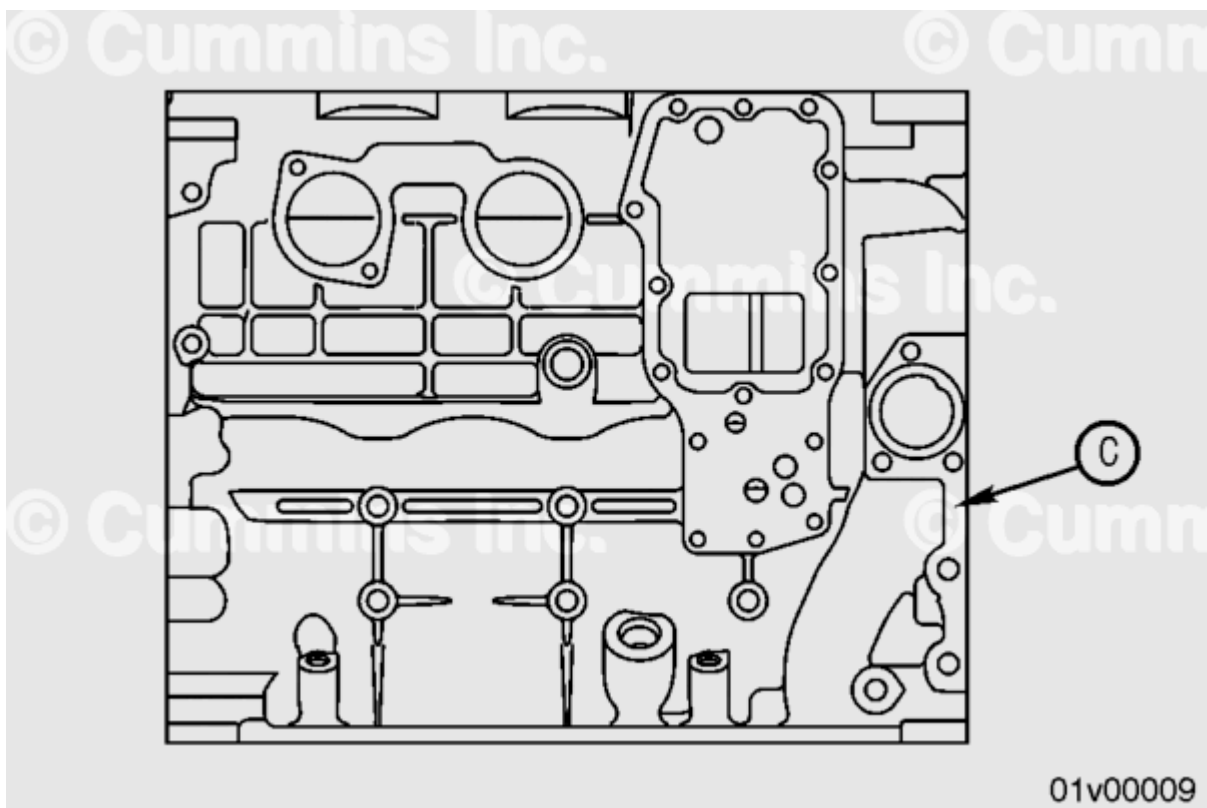
Right Side View - ISB, ISD, ISBe, and B-4 Cylinder
