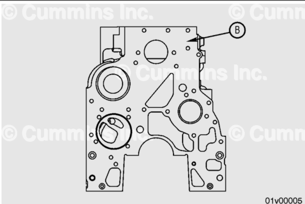
Front View - ISB, ISD, ISBe, and B Series-4 Cylinder
