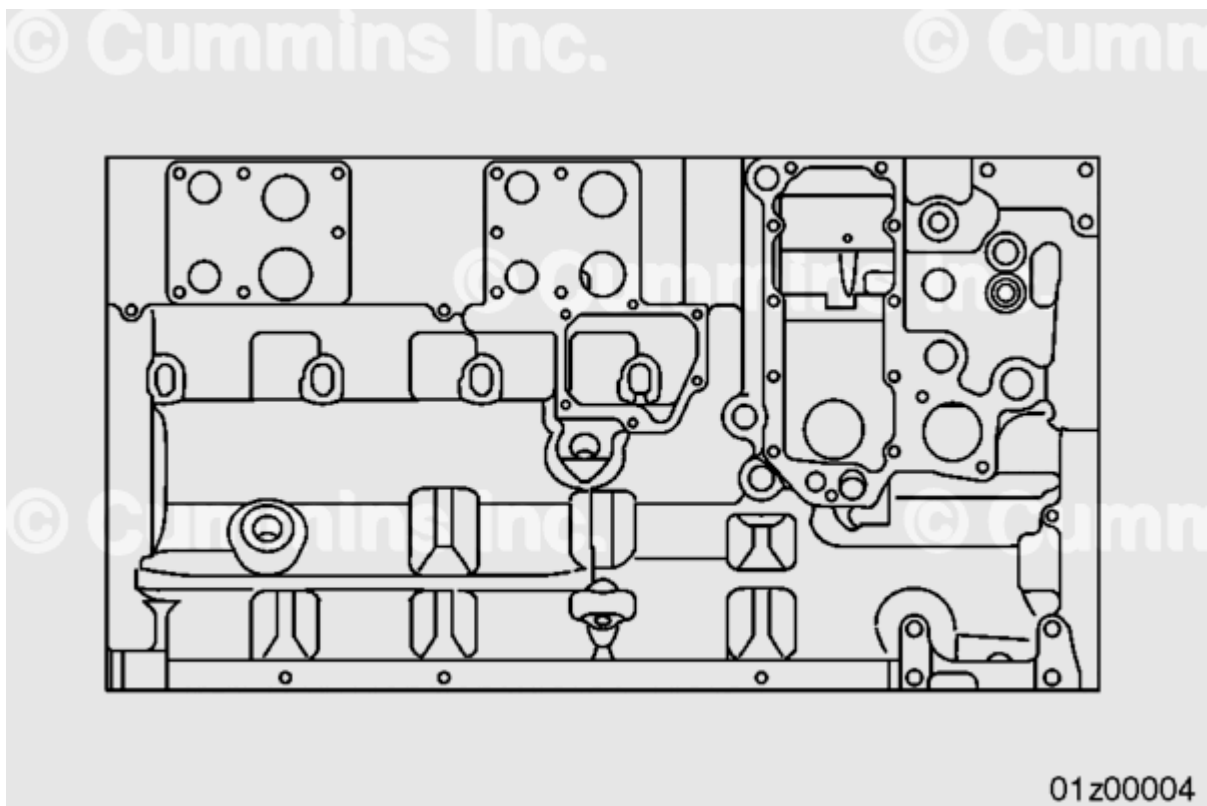
Rear View -ISC, ISL, QSC, and QSL
