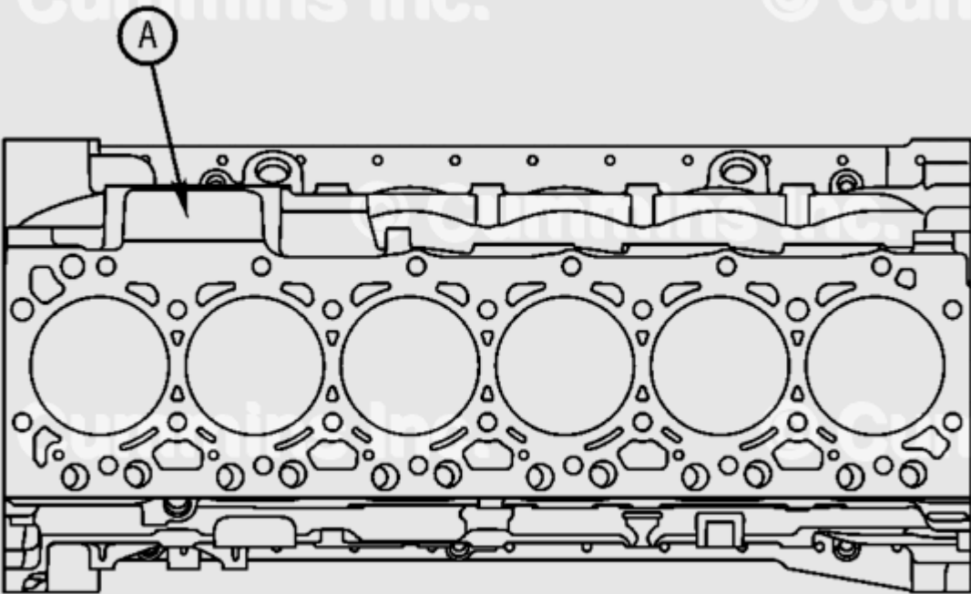
Left Side View - QSB, ISB, ISD, ISBe, and B
