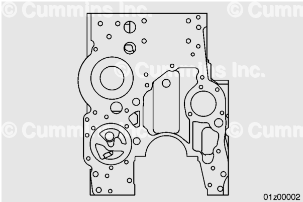
Front View - ISC, ISL, QSC, and QSL
