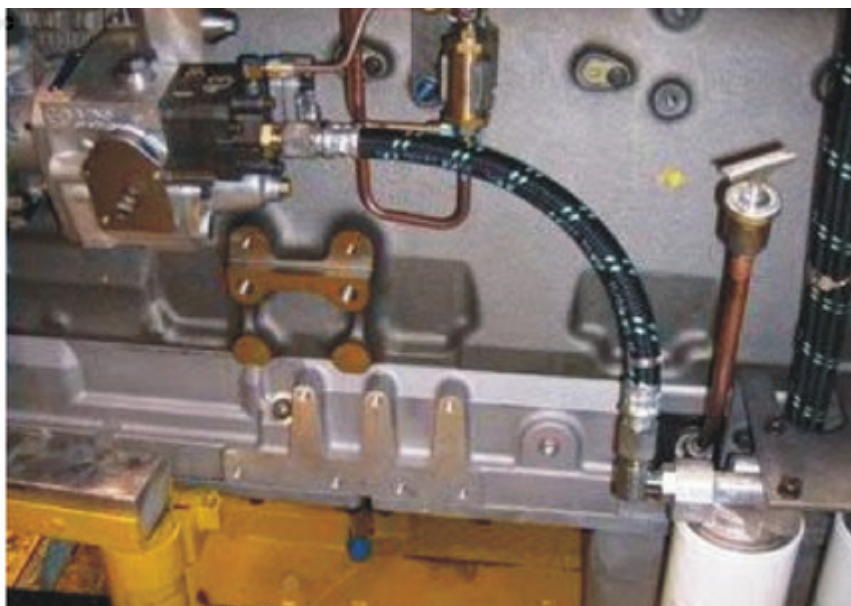
Figure 3, Alternate Fuel Filter Mounting Location
