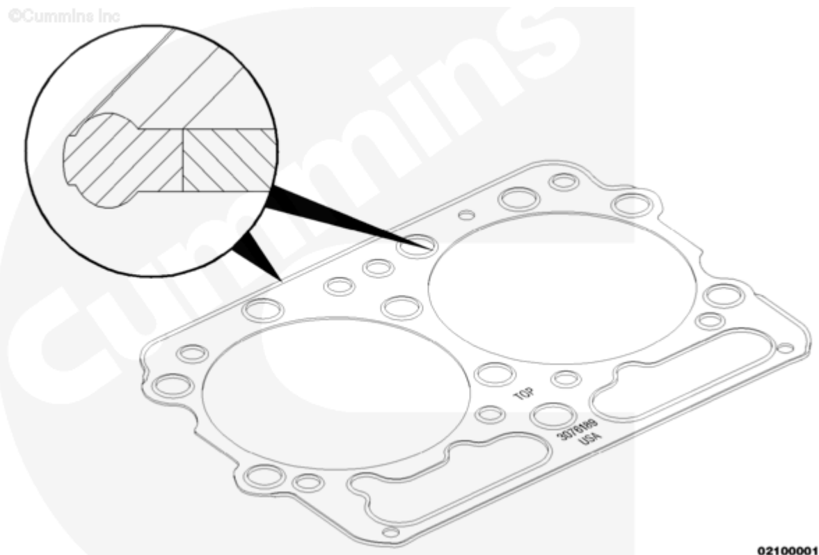
Figure 1, New cylinder head gasket.
