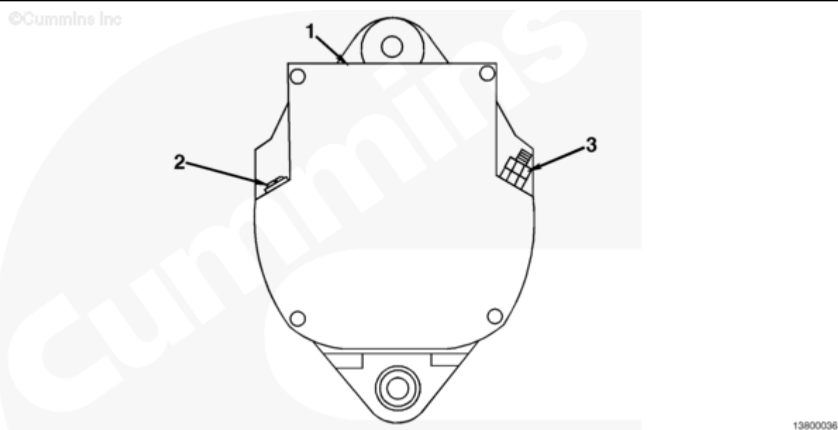
Figure 3, 30SI Alternator
