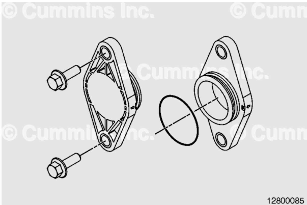
Figure 2. New Composite Compressor Cover with Flange Head Capscrews
