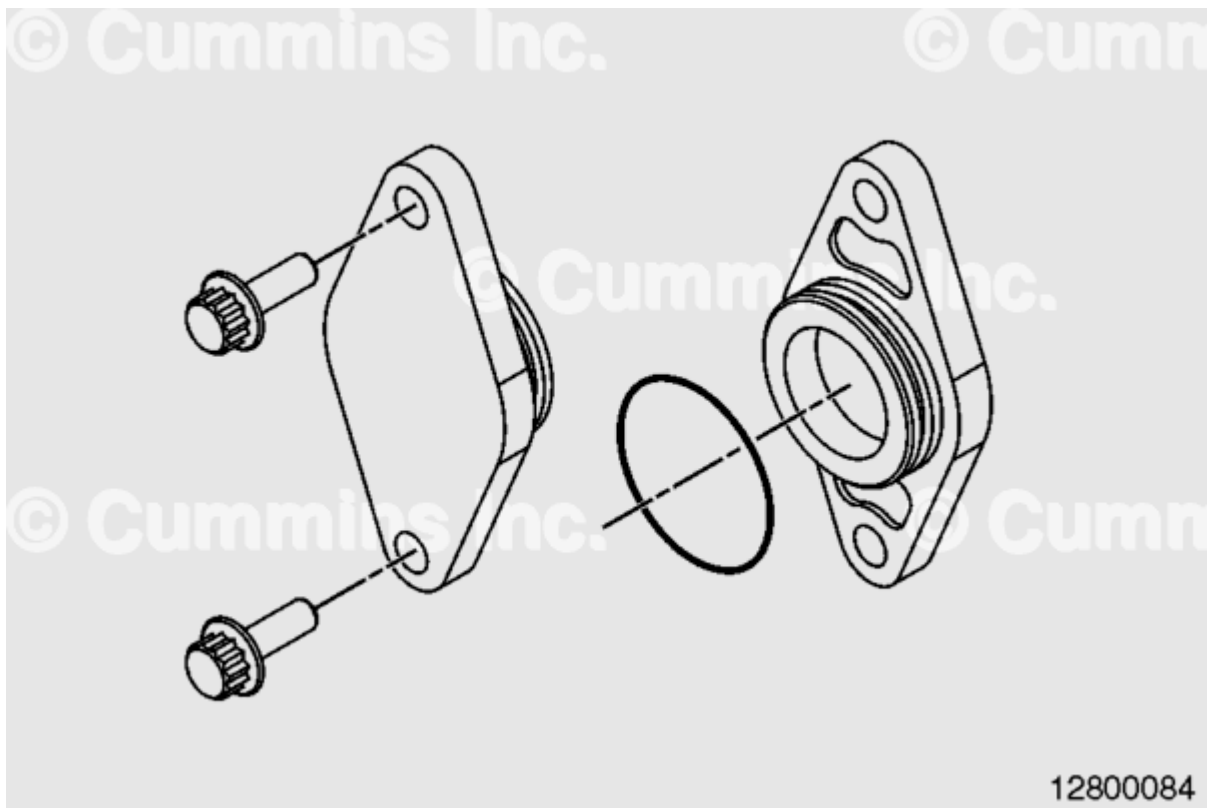
Figure 1. Existing Aluminum Compressor Cover with 12 Point Capscrews
