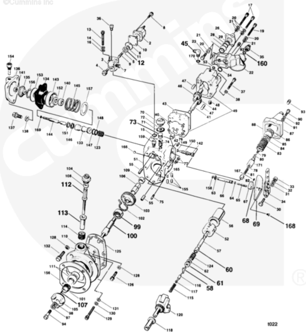
PT (TYPE G) AFC FUEL PUMP PARTS
