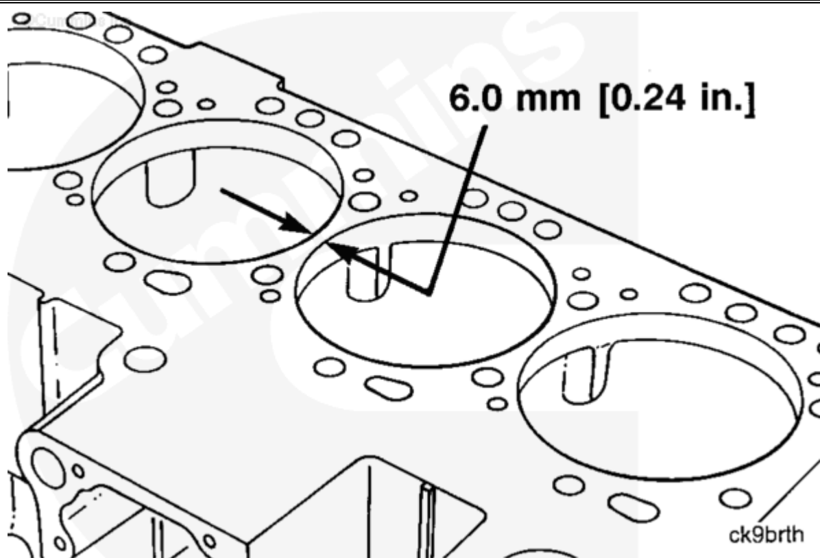
Thick-Wall Cylinder Block
