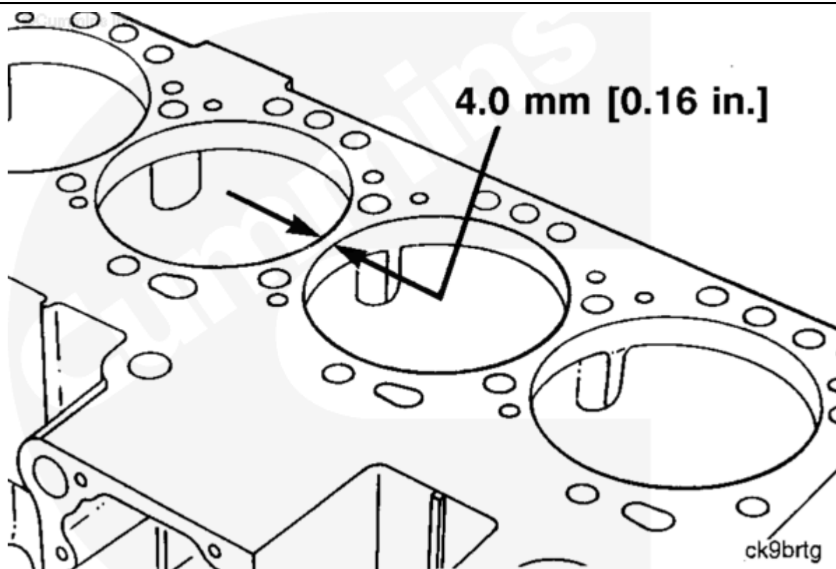
Thin-Wall Cylinder Block
