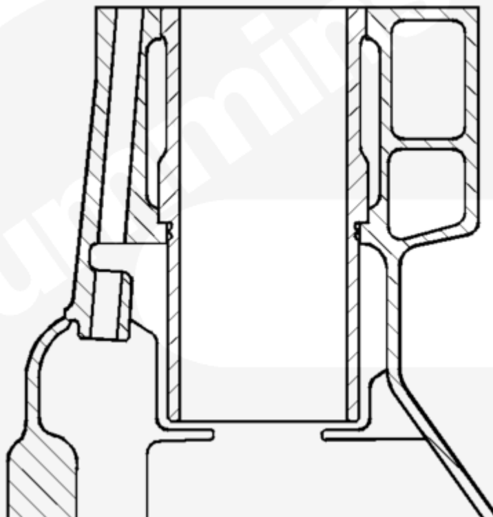
Fig. 1, Old Liner/Old Block
