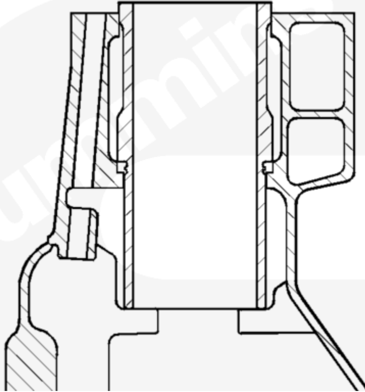
Fig. 3, Old Liner/New Block
