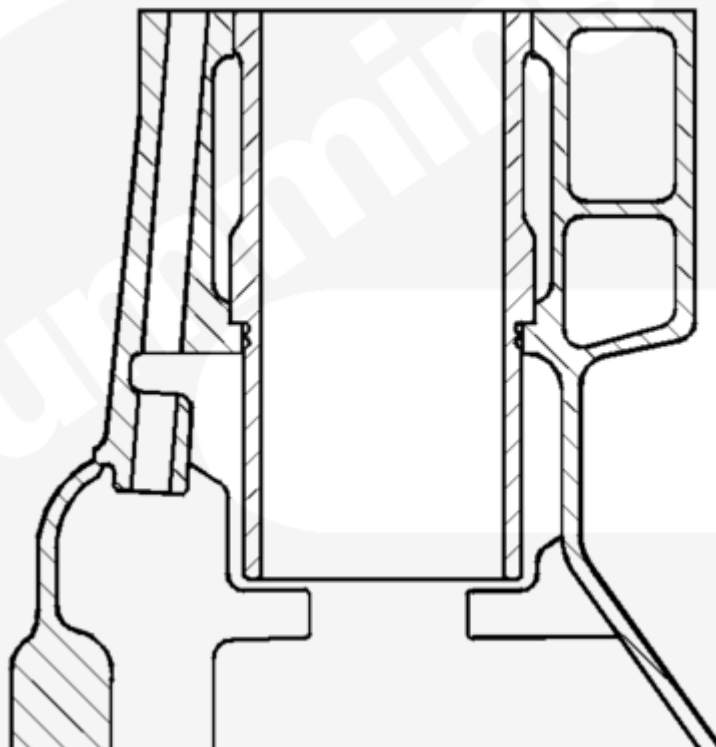
Fig. 2, New Liner/New Block
