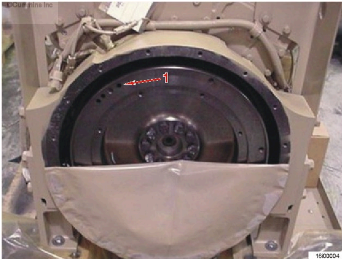
Picture 2: Holes drilled in the correct location (Surface 1).
