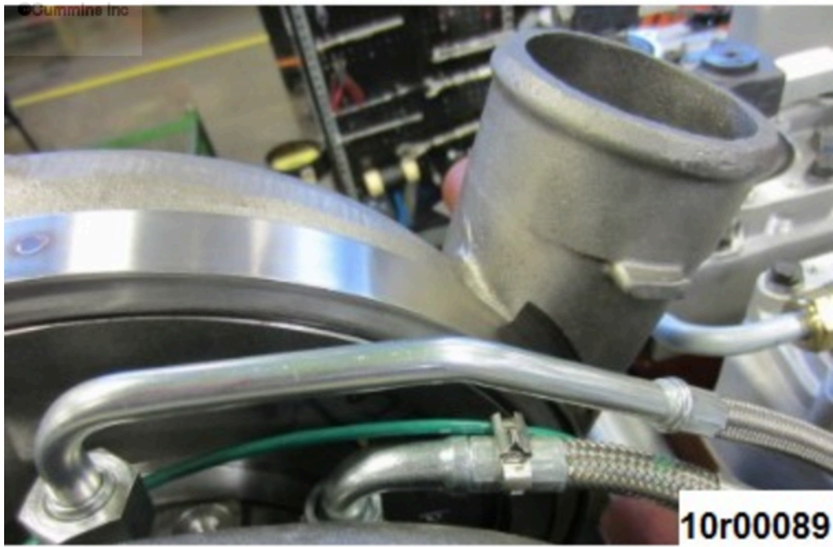
Figure 2, New Turbocharger Oil Supply Line Installed On Engine
