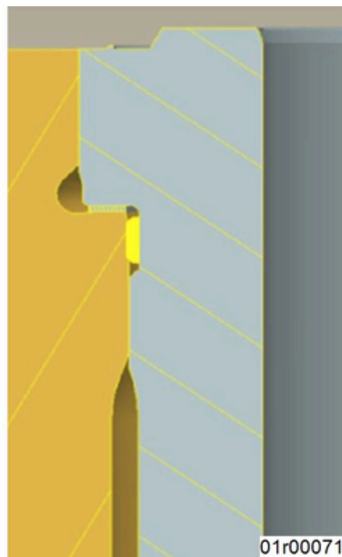
Figure 2, Existing Cylinder Liner and Upper Crevice Seal Installed in Cylinder Block
