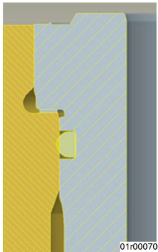
Figure 1, New Cylinder Liner and Upper Crevice Seal Installed in Cylinder Block
