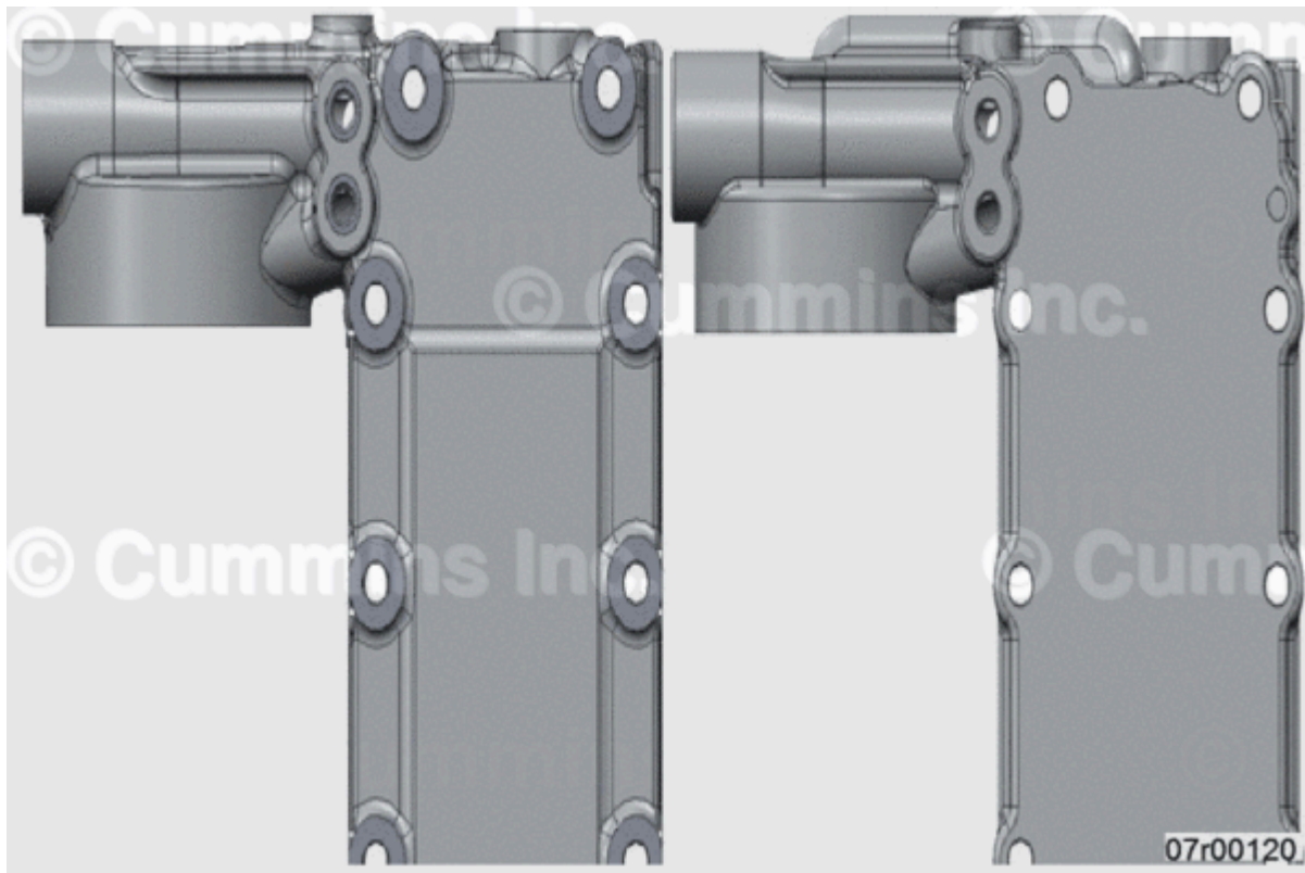
Figure 1: Left: Lubricating Oil Filter Head. Right: Existing Lubricating Oil Filter Head.
