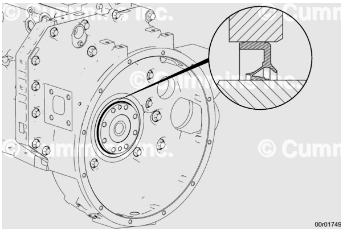
Figure 2, Lip Crankshaft Seal
