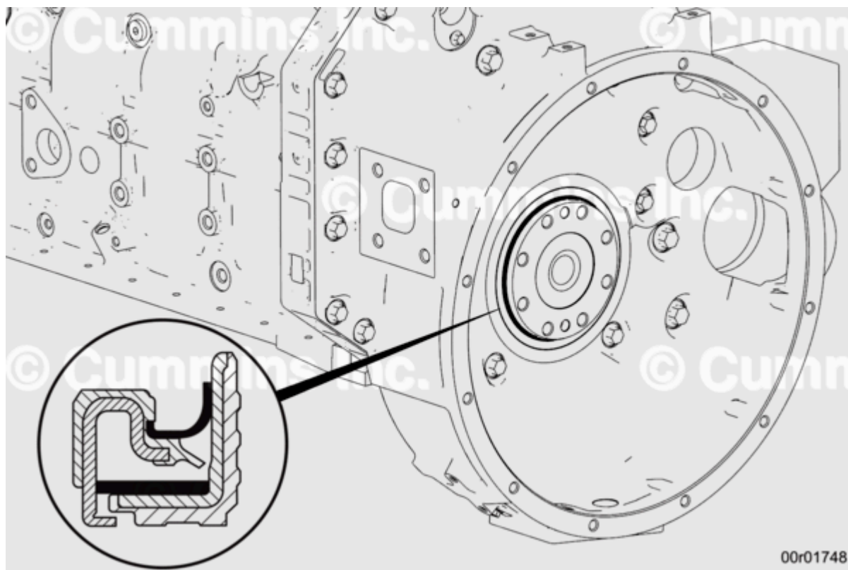
Figure 1, Unitized Crankshaft Seal
