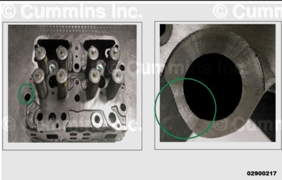
Figure 1, Acceptable Recon® Cylinder Head Mounting Hole Salvaging
