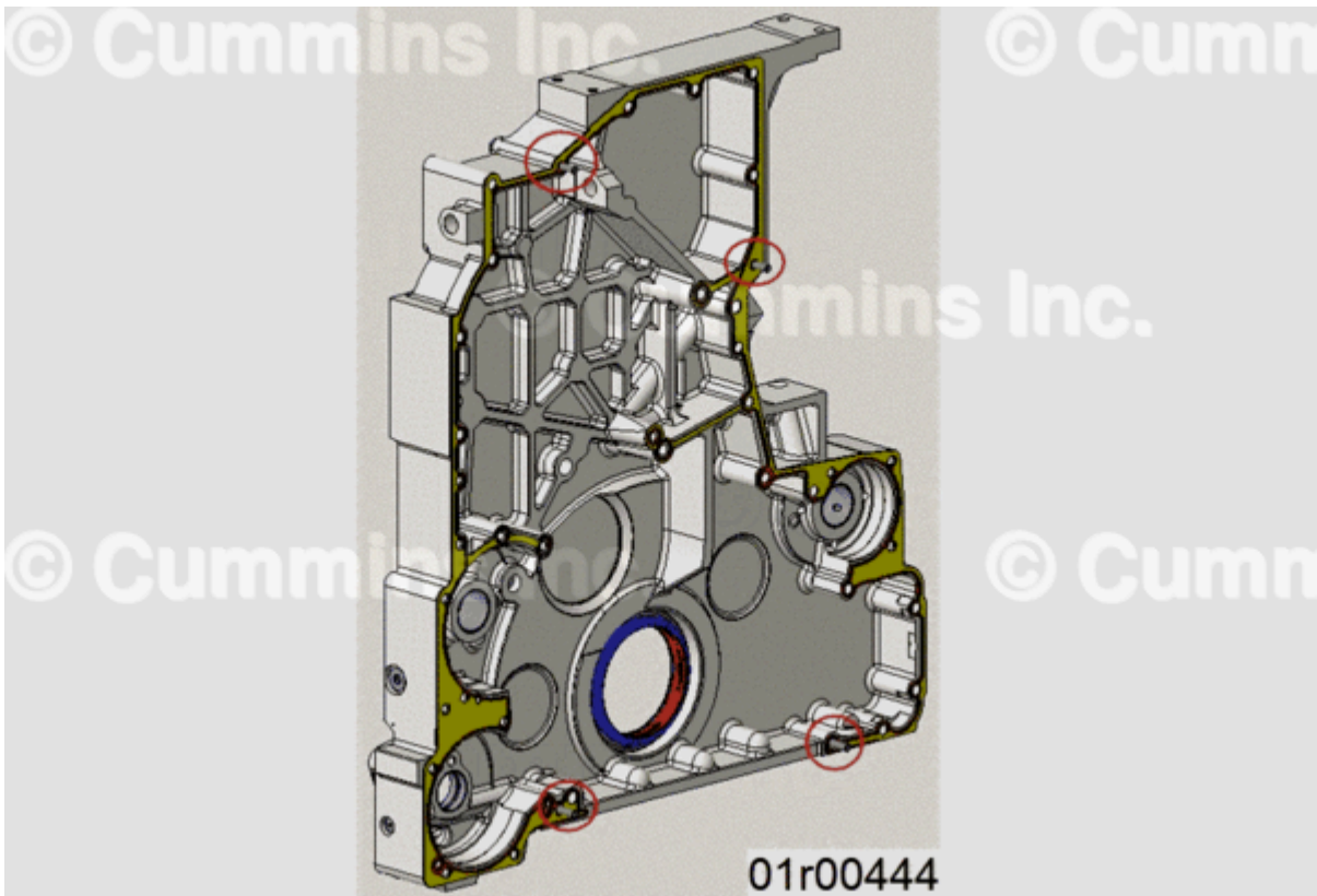
Figure 1, Front Gear Cover Gasket Rubber Retention Locations.
