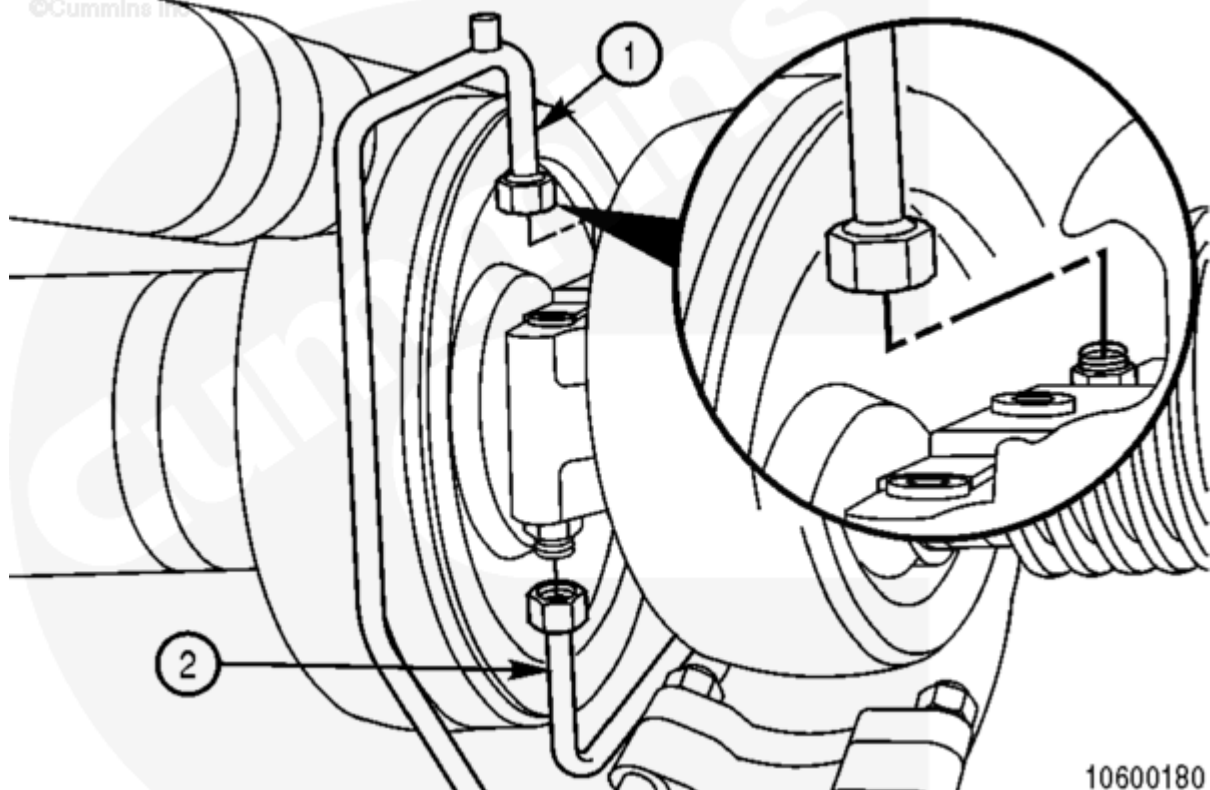
Fig. 1, Turbocharger Coolant Supply and Drain Hose Mounting (high pressure)
