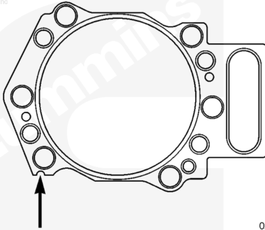
Figure 4, Oversize Gasket Notch
