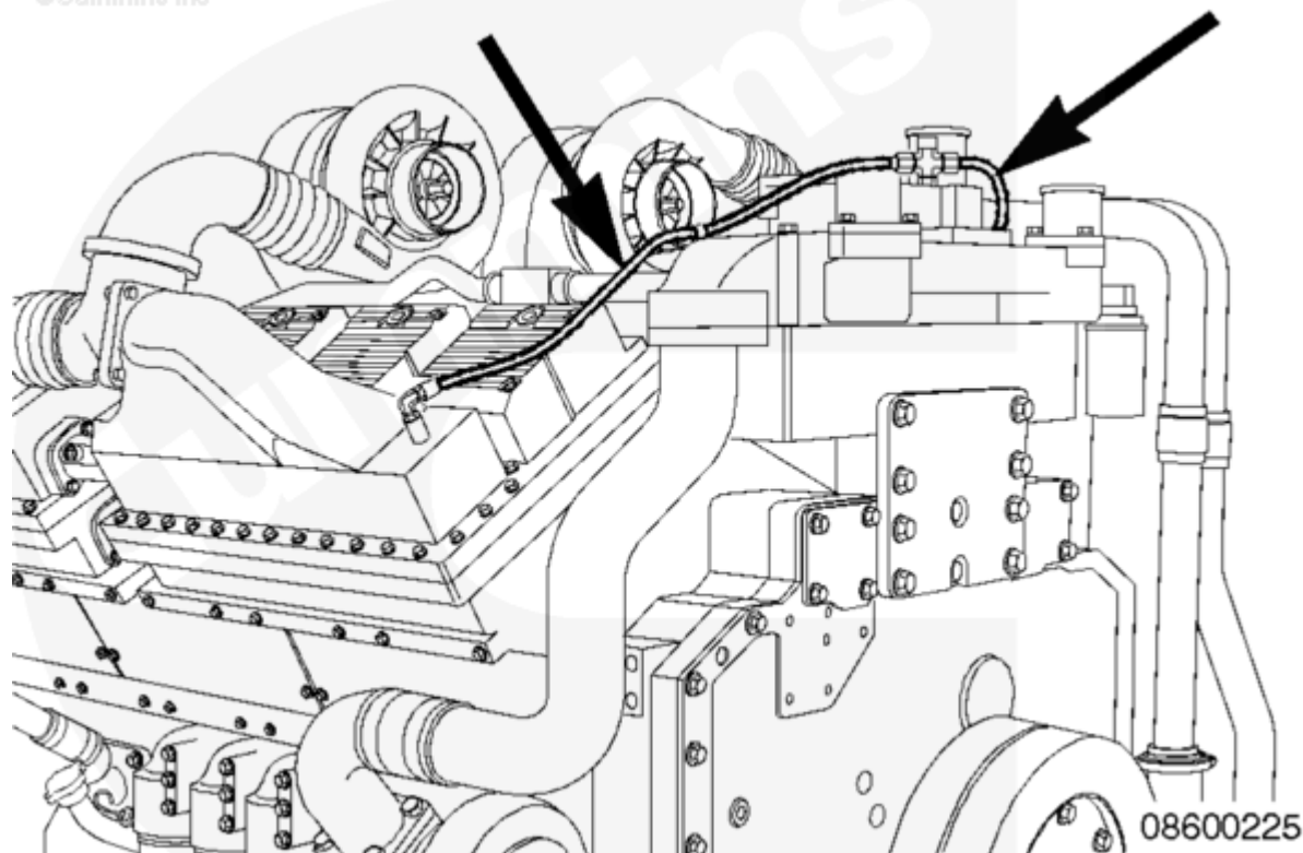
Old Type 1 Installation with Aftercooler Vent Line Locations
