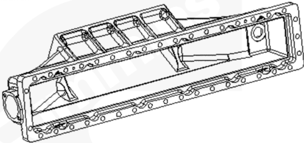
New Aftercooler Cover (external view)
