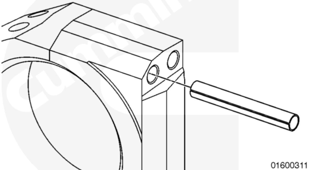
Spring Dowels (Exploded View)
