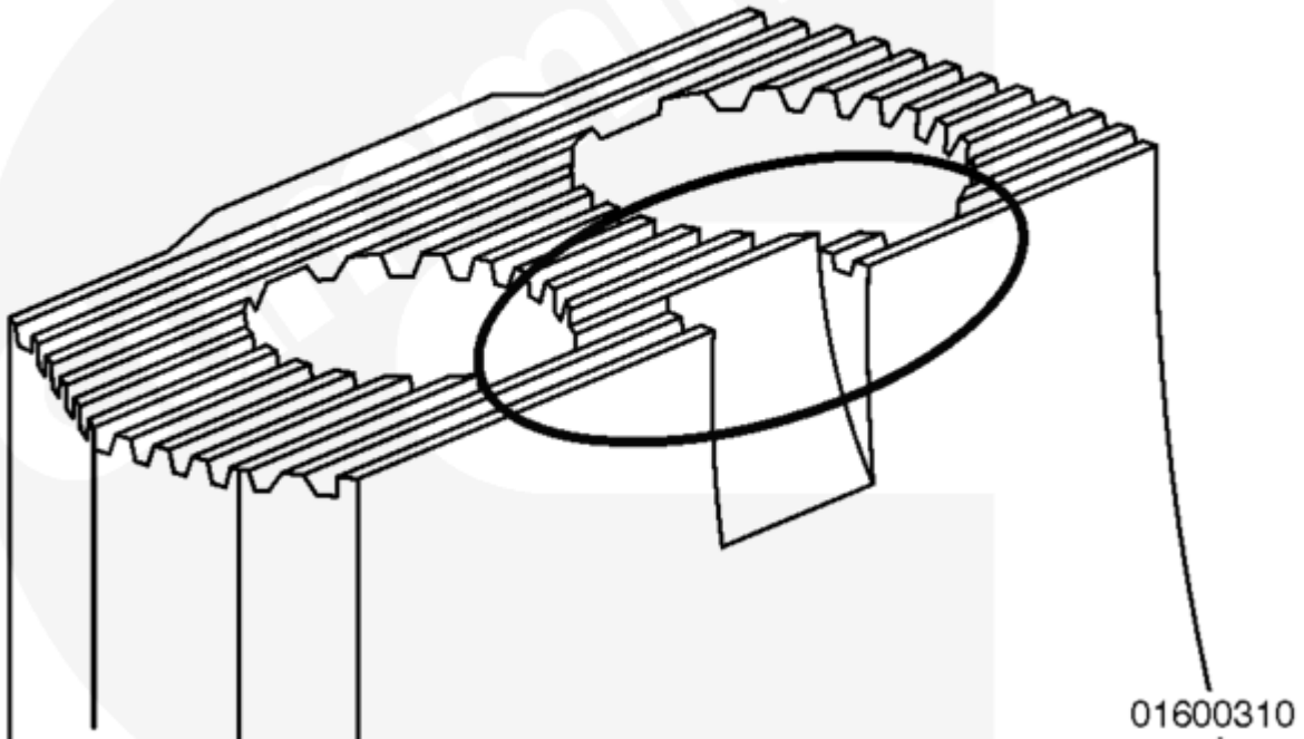
Improved Serration Surface
