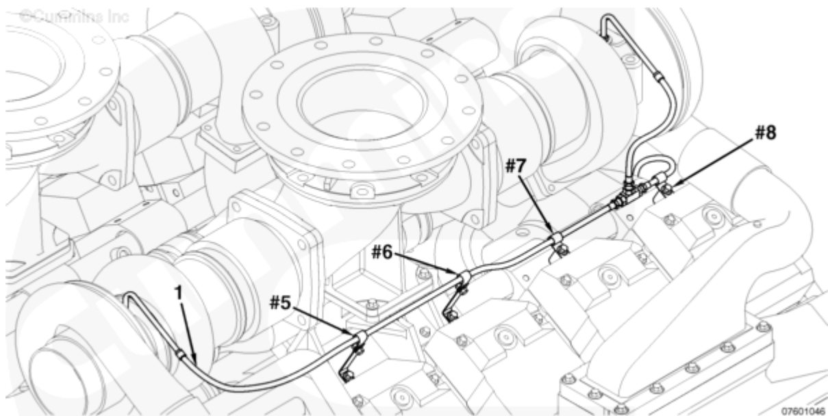
Figure 3, Left Bank, Clips at Number 5 and Number 6 are extended, clips at Number 7 and Number 8 are short.
