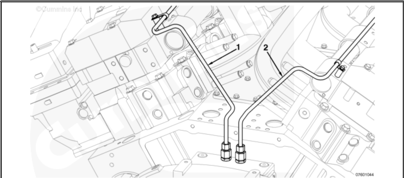
Figure 1, Old arrangement with oil supply tubes from the flywheel housing.
