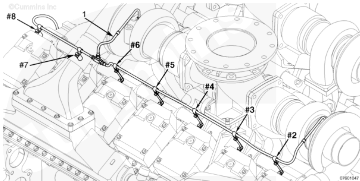
Figure 4, Right Bank, Clips at Number 2 to Number 6 are extended, Clips at Number 7 and Number 8 are short.
