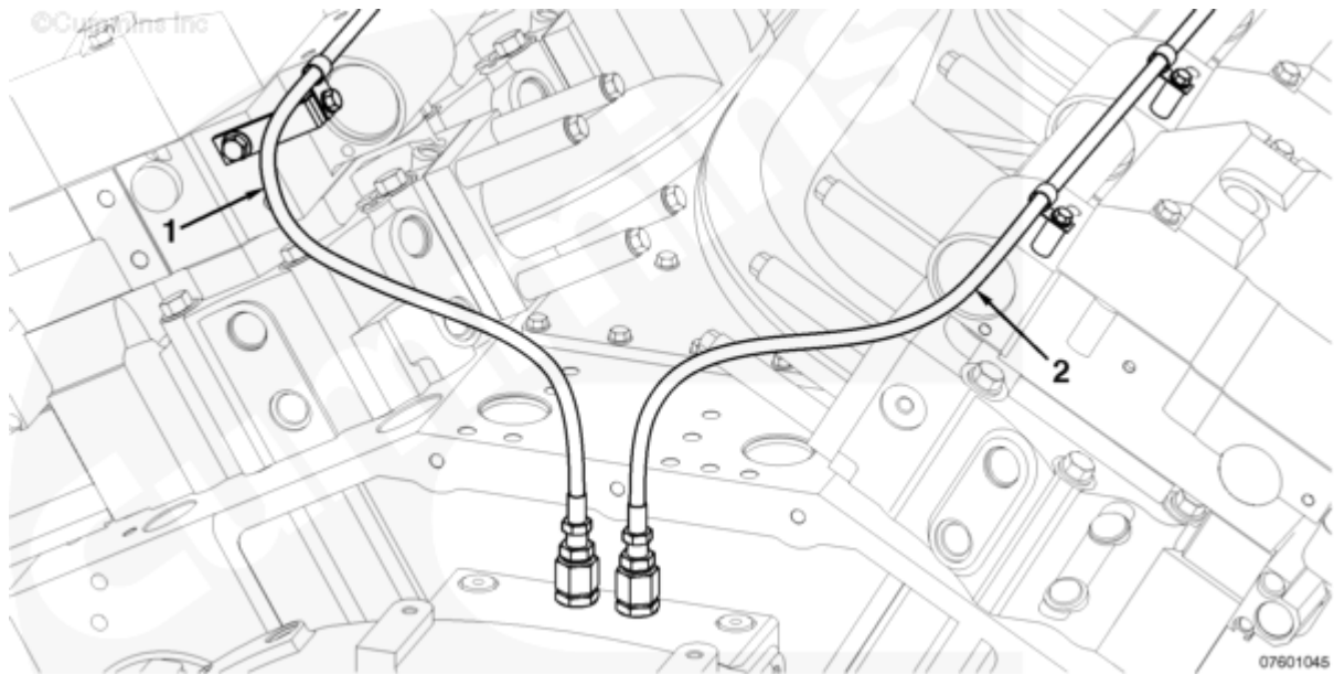
Figure 2, New arrangement with oil supply hoses from the flywheel housing to tees
