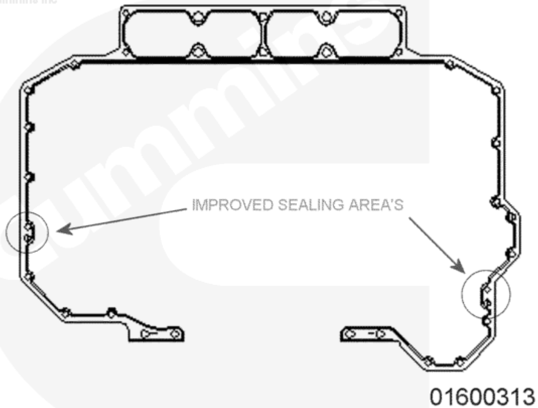
Figure 1 New Gear Cover Gasket, Part No. 4100983.
