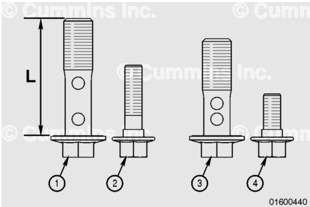
Figure 3, Old Banjo (1) and Center Bolt (2), New Banjo (3) and Center Bolt (4)
