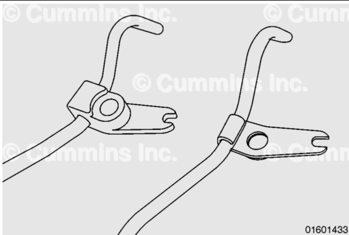
Figure 1, Old Long Piston Cooling Nozzle (left) and New Long Piston Cooling Nozzle (right)
