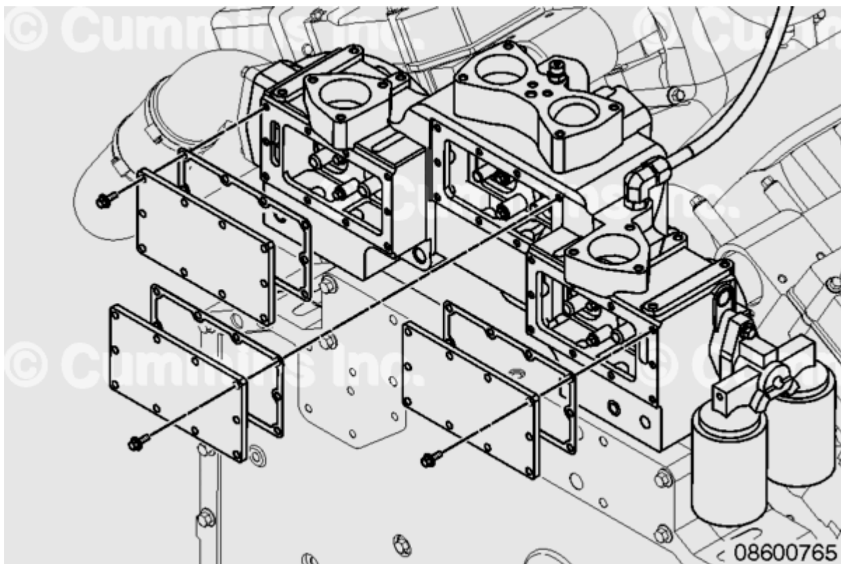
Figure 1, New Thermostat Housing.
