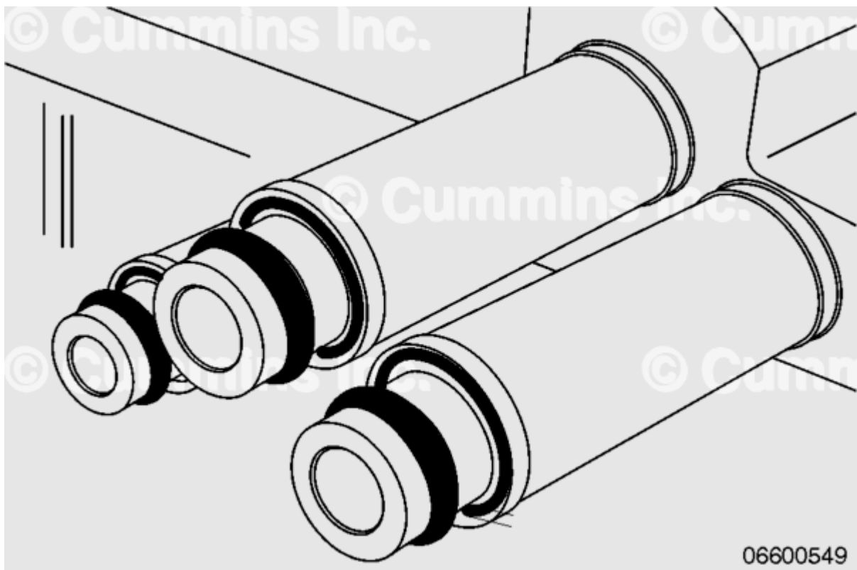
Fuel Transfer Tube o-rings and dust seals
