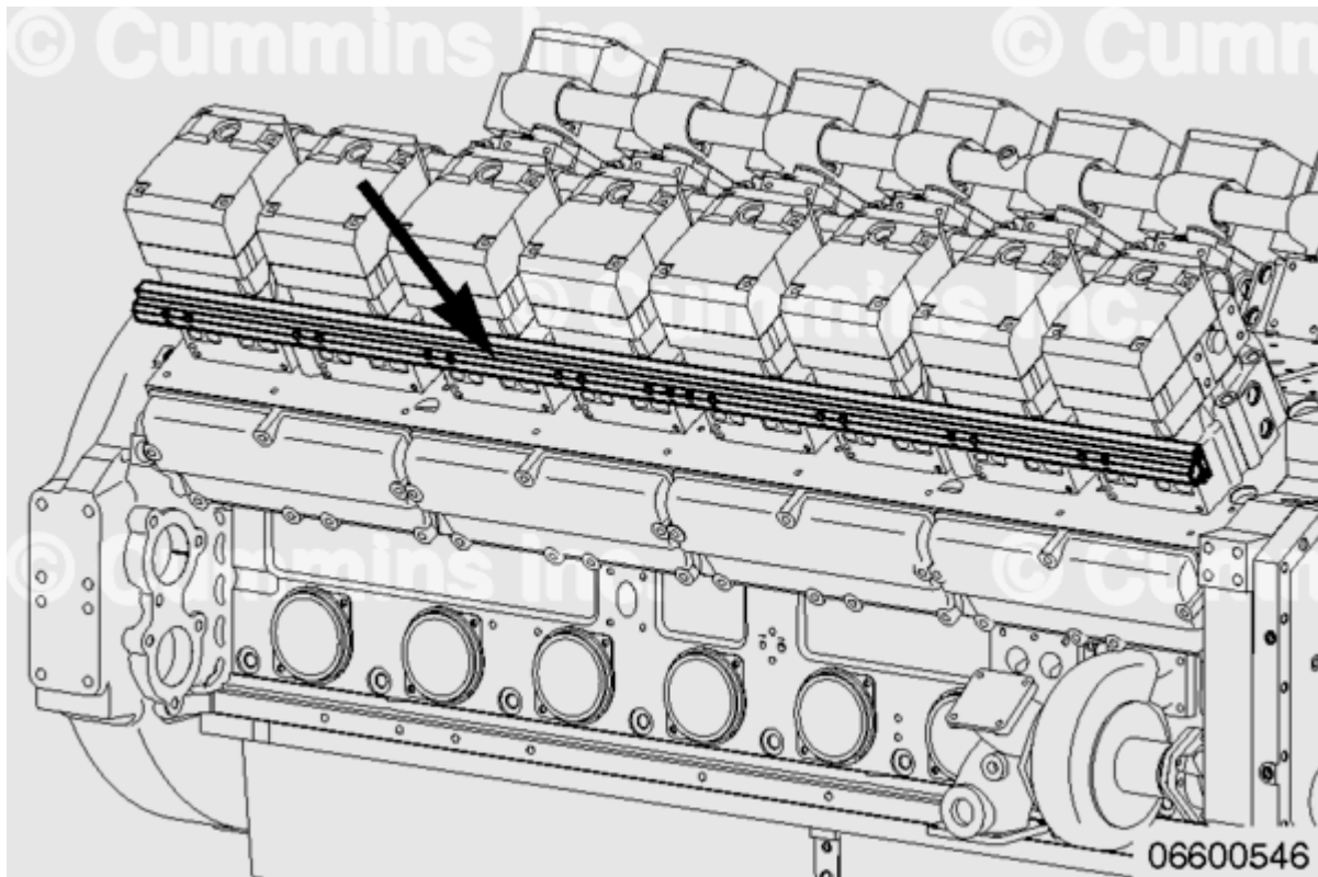
One Piece Fuel Manifold
