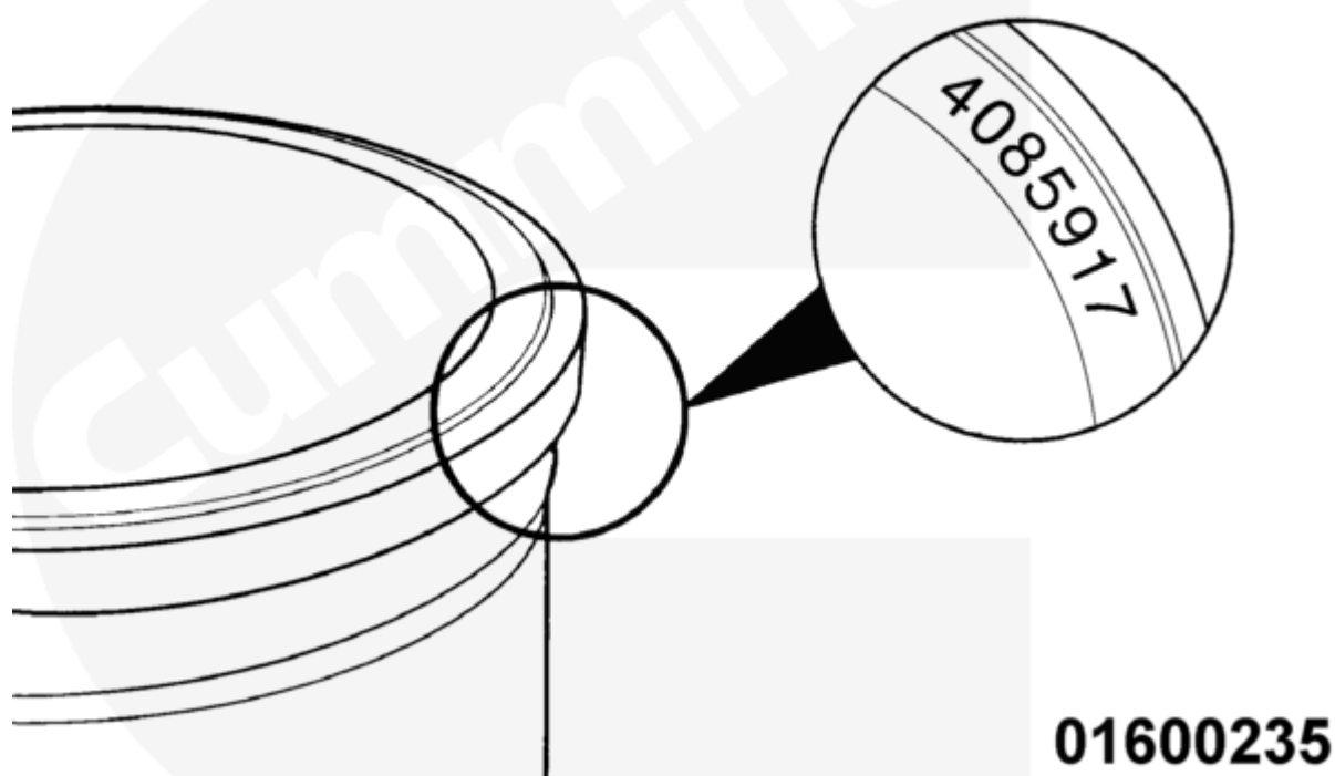
Fig. 1. Cylinder Liner Part Number Location
