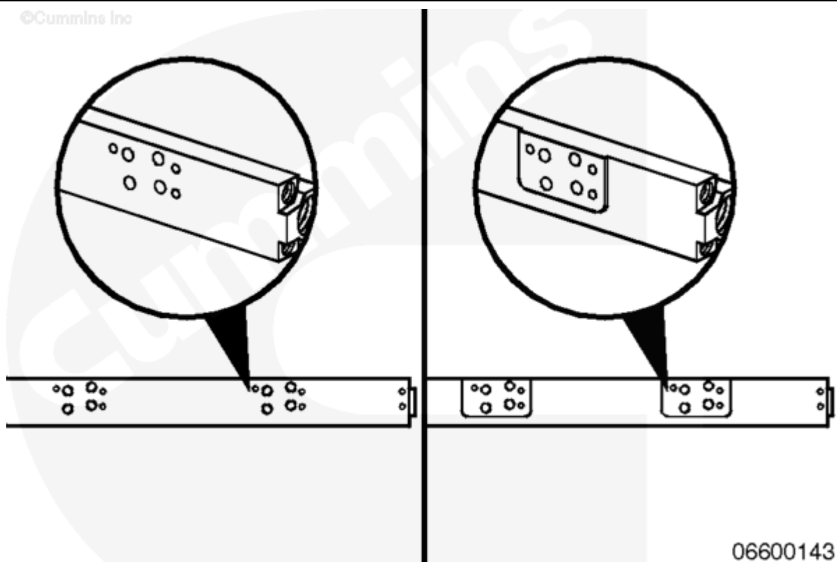
Figure 1, Old and New Style Fuel Manifold
