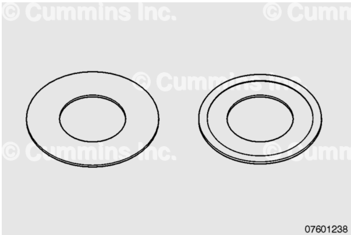
Old Paper Oil Cooler Stud Gasket, Part Number 3630969 (left) and New Edge-mounted Oil Cooler Stud Gasket, Part Number 3637730 (right)
