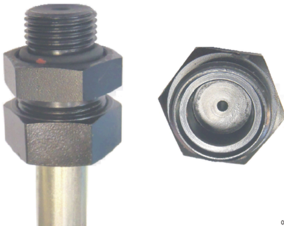
Figure 1: Outlet Restricted Coupling, Part Number 3649824
