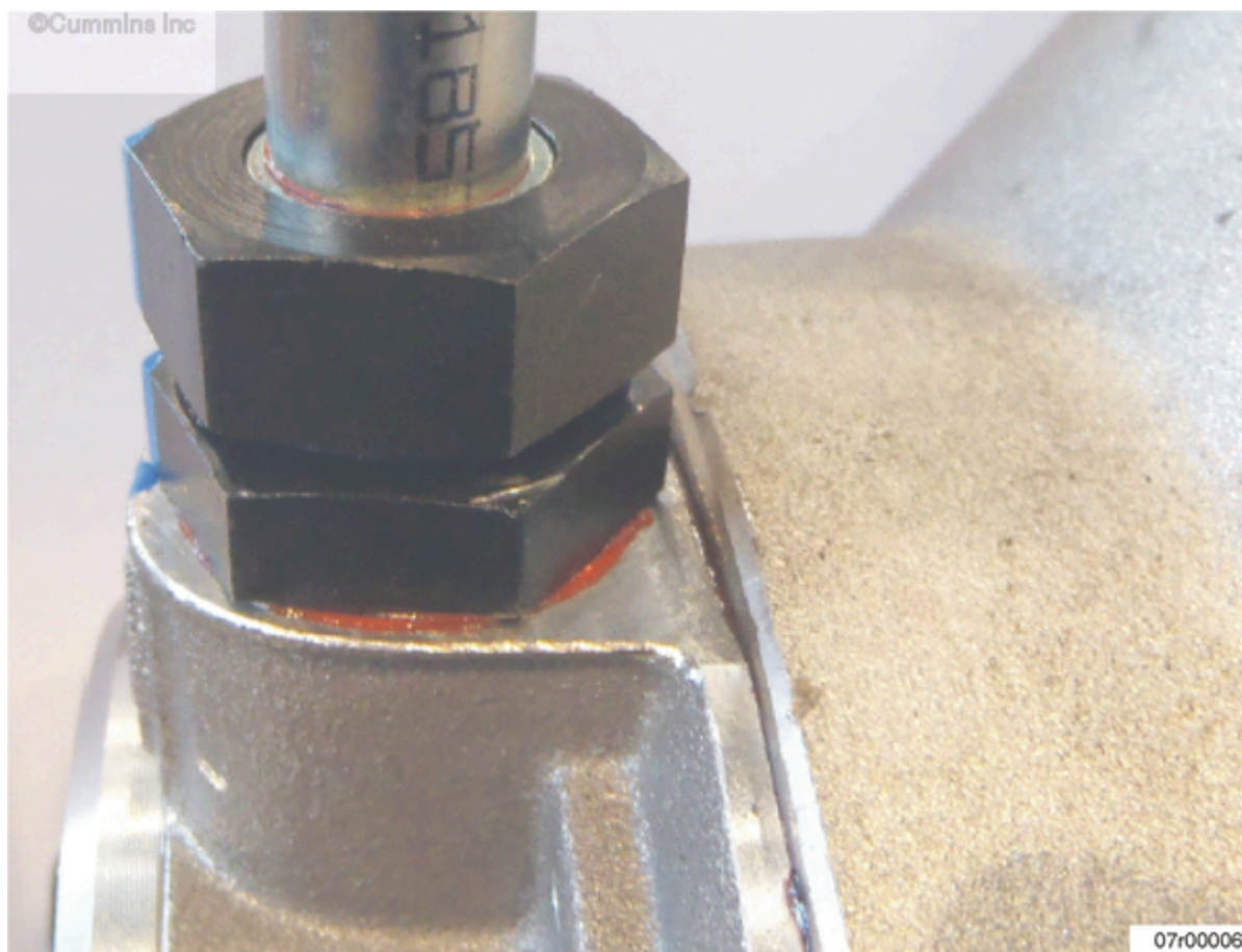
Figure 2: Location of Outlet Restricted Coupling
