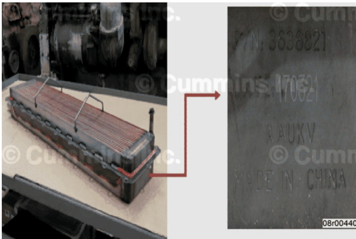
Figure 3, Intercooler Core Part Number Identification
