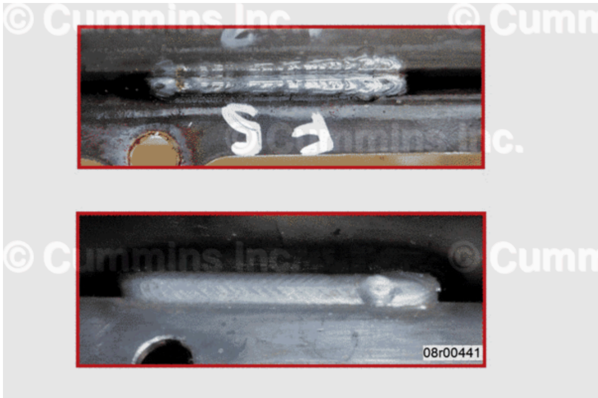
Figure 1, Top: Manual Weld Malfunction. Bottom: New Robotic Weld.
